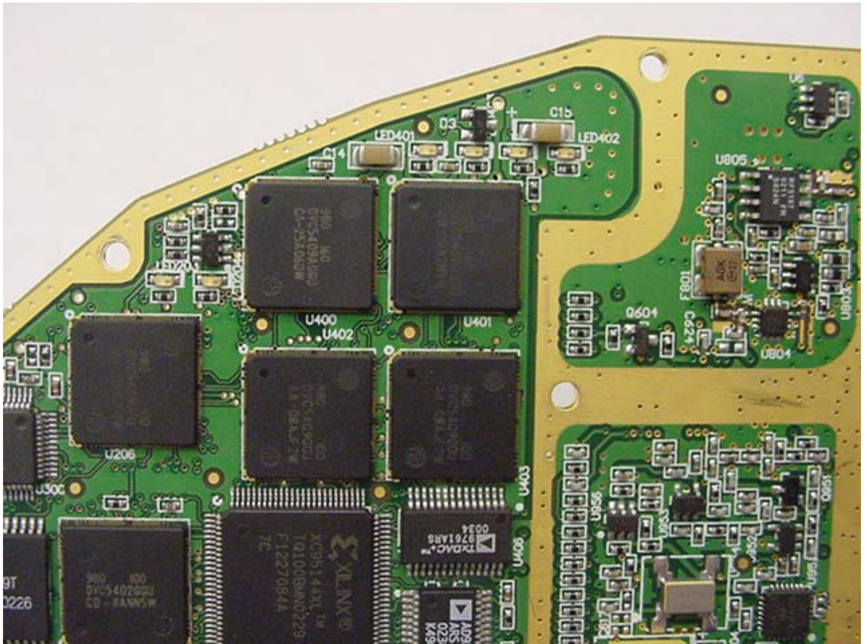
USB Populated Board
