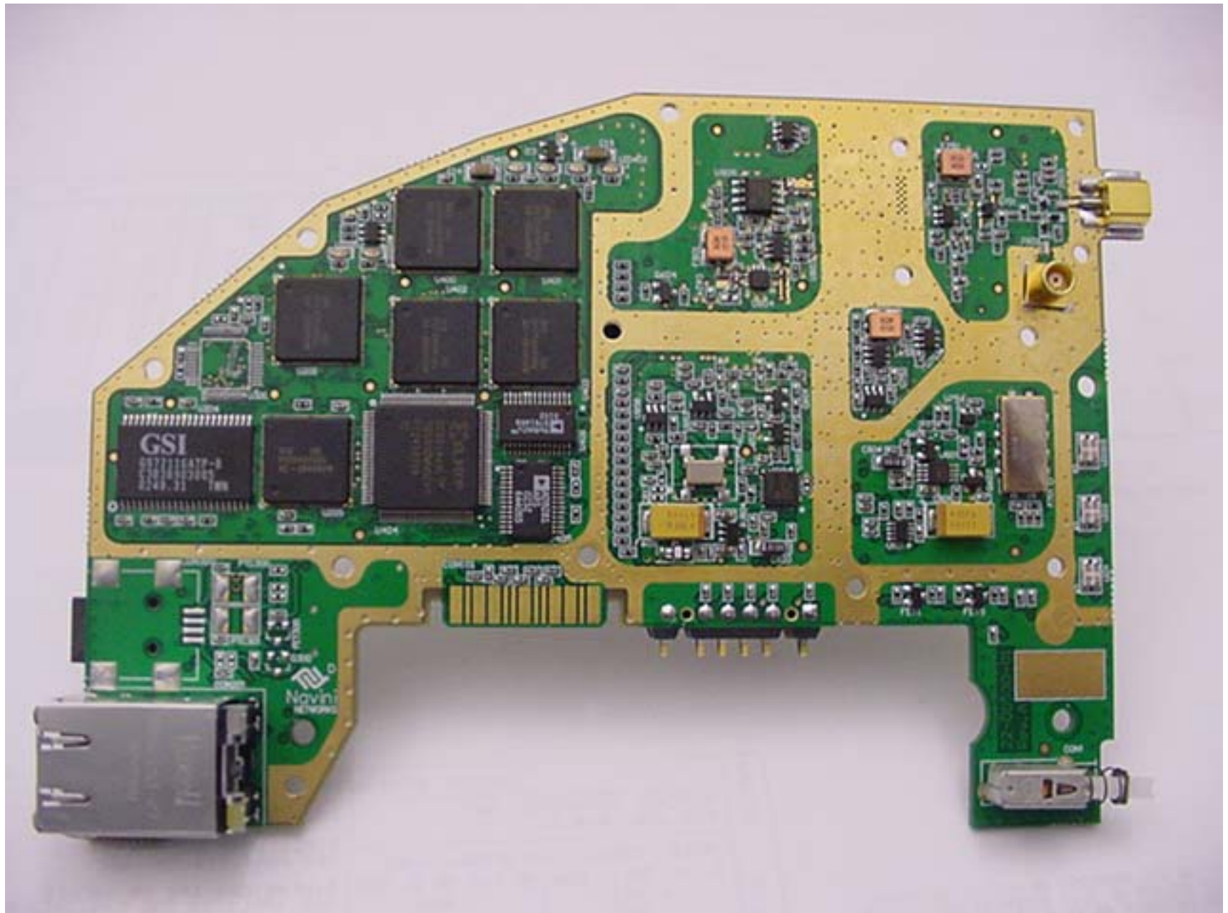
Ethernet Populated Board
