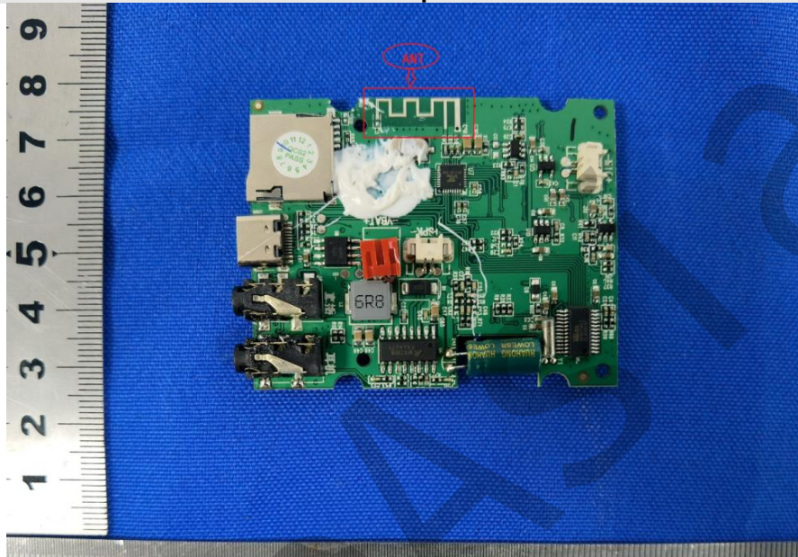
Antenna Requirement
