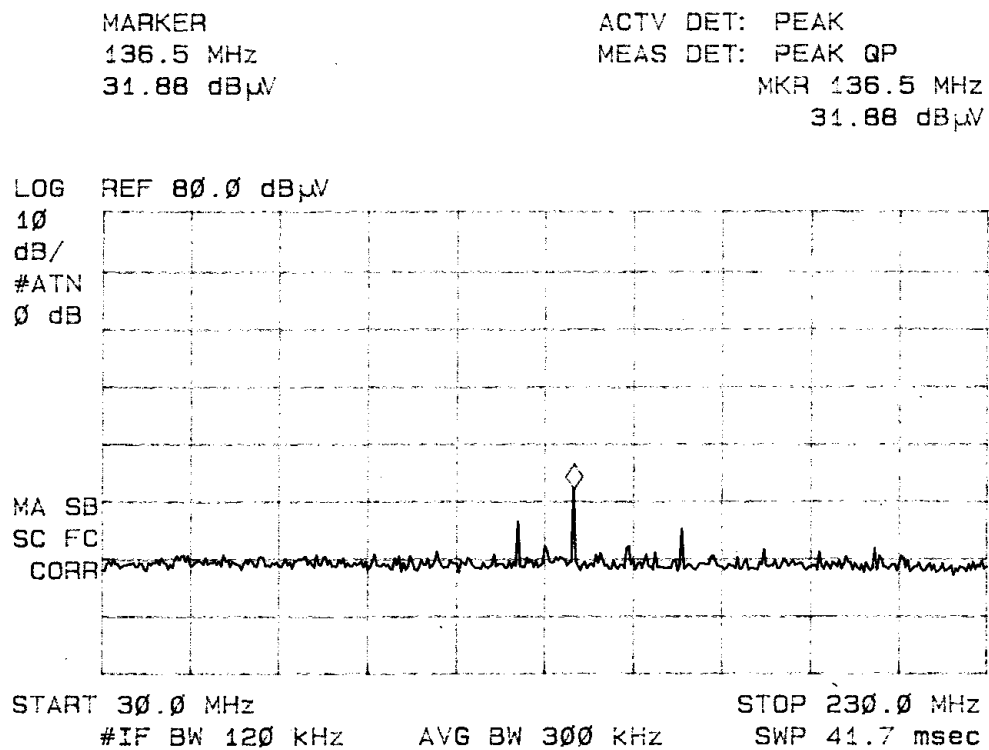
Figure 1. Radiated Emissions taken at 1 meter in screen room.
