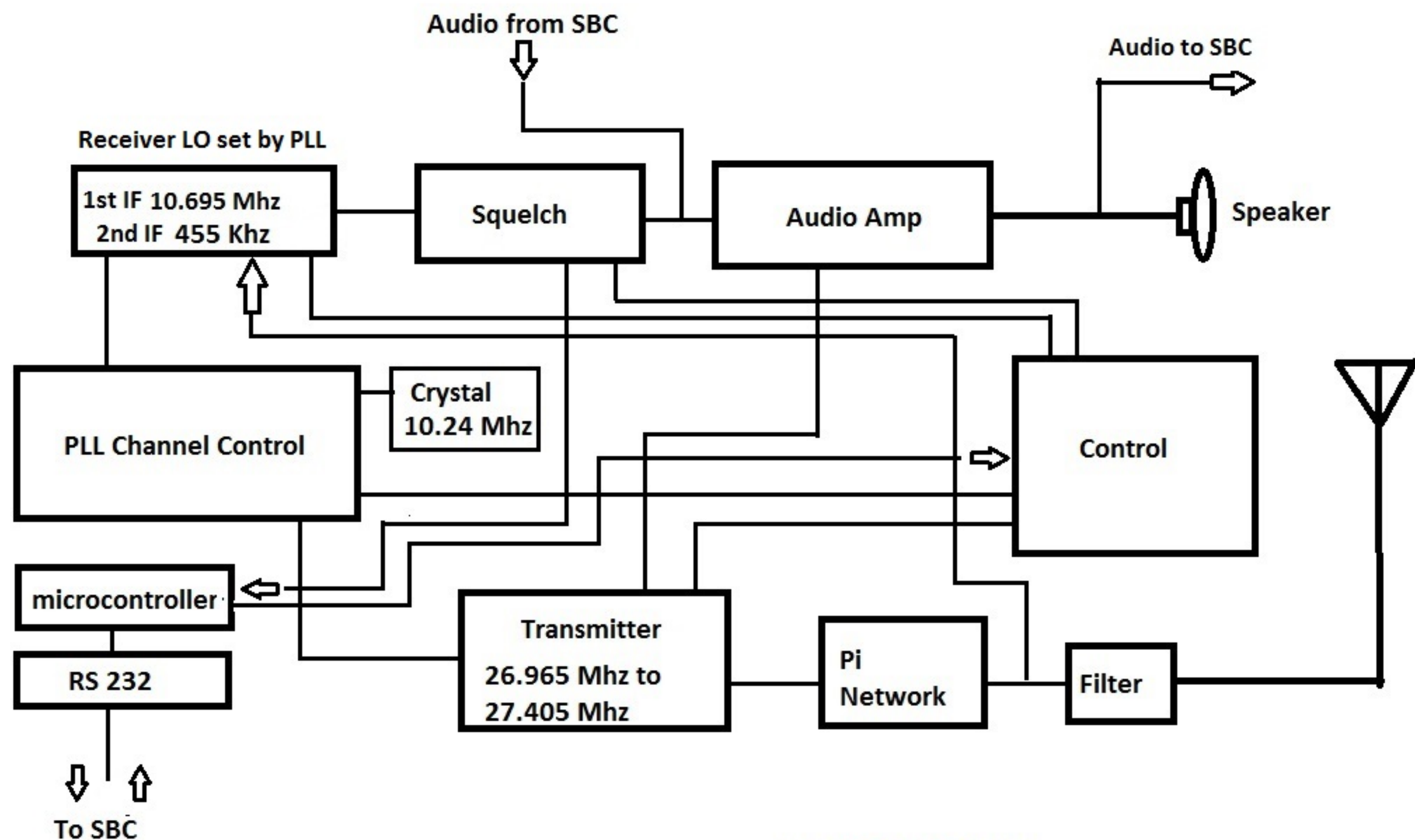
RBS-CB Block Diagram Clenney Communications, Inc.
