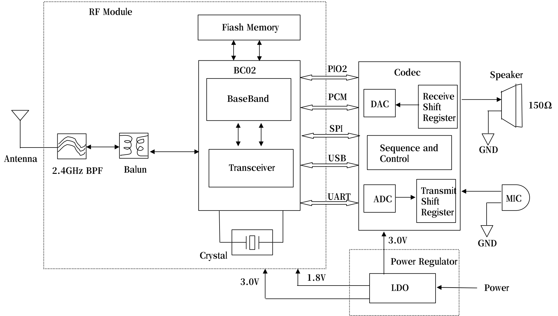
GBH-200H (Headset) Block Diagram
