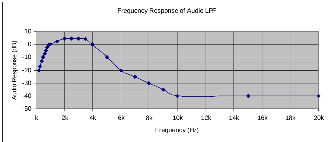
Figure 3 Frequency Response of Audio low Pass Filter.
