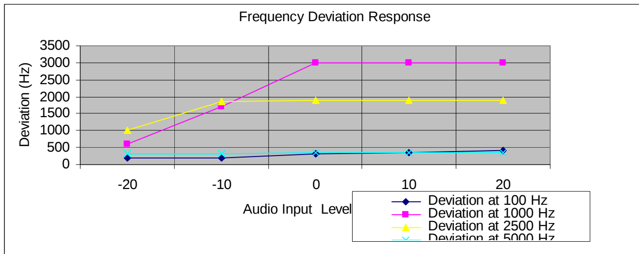
Figure two Deviation Characteristics.
