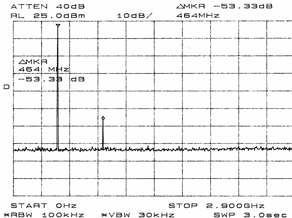
Figure five Emissions at Antenna Terminal
