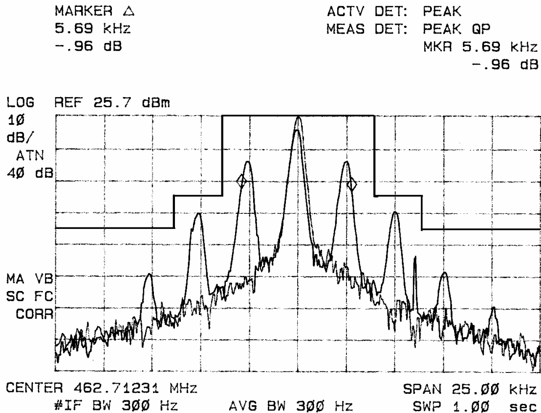
Figure four Occupied Band Width. Data taken with 6dB attenuation at output of 1.5 Watt (31.7 dBm) transmitter.
