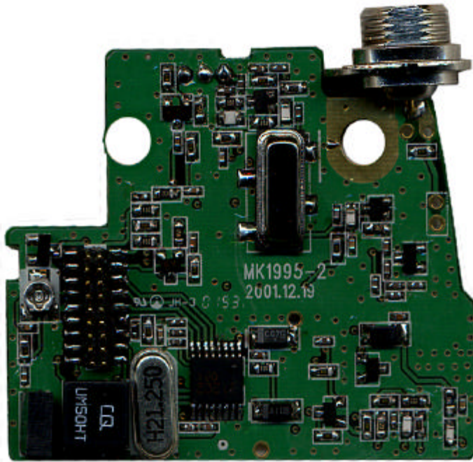
RF printed circuit board bottom.
