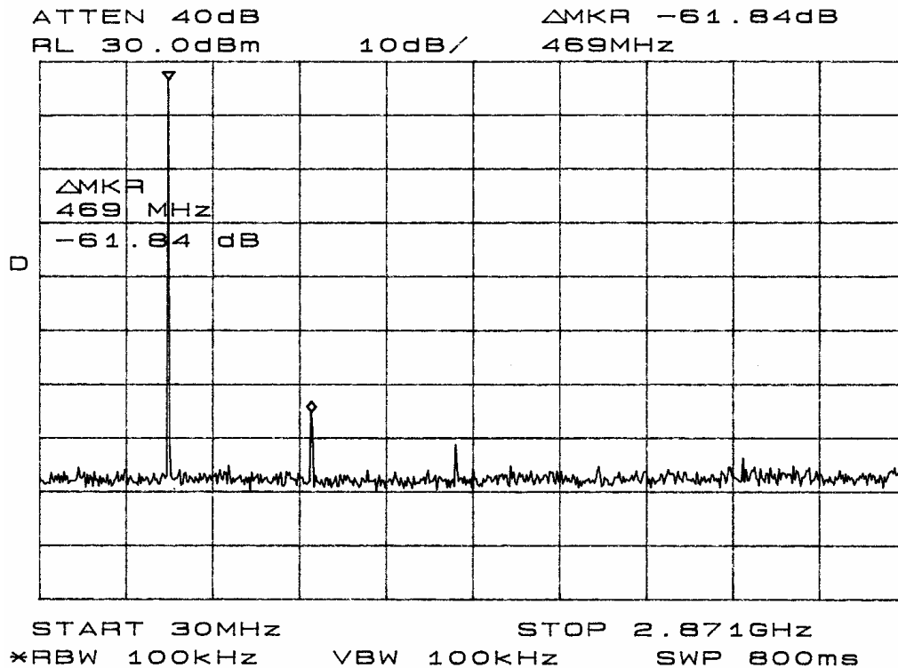
Figure 7: Emissions at Antenna Terminal (467.55 MHz)
