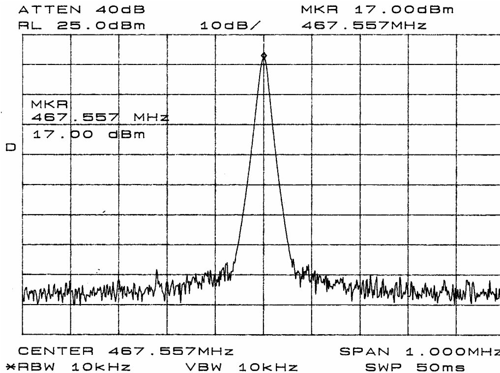
Figure 1A: Power Output Channel 467.55 (with 10dB attenuation)
