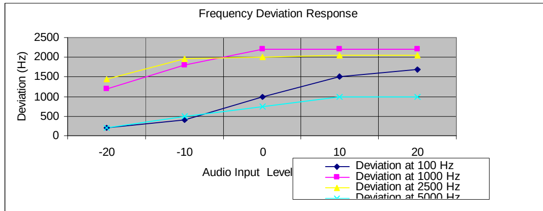
Figure 3: Deviation Characteristics.
