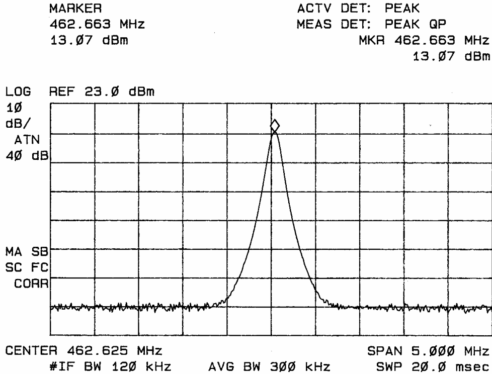
Figure 1: Power Output Channel 462.625 (2-Watt High Power)
