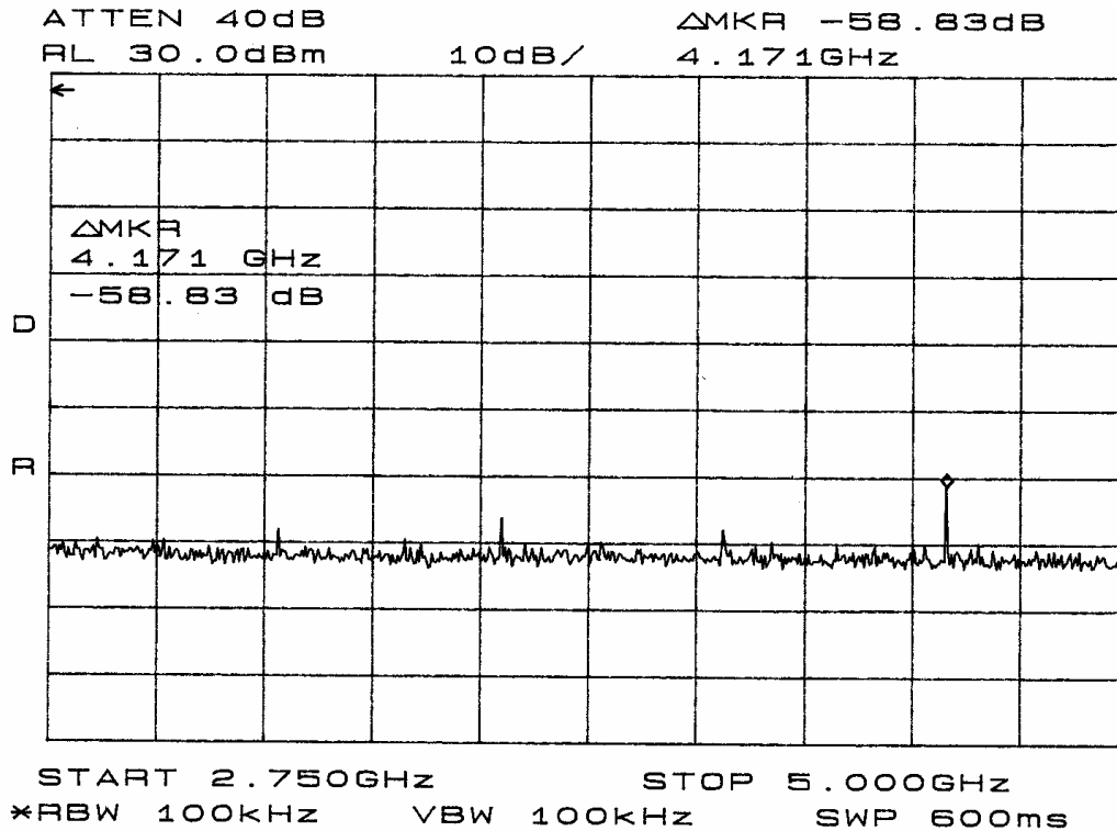
Figure 6A: Emissions at Antenna Terminal
