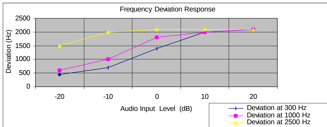
Figure 3: Deviation Characteristics.
