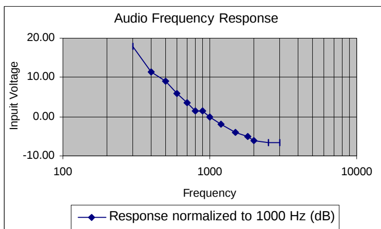
Figure 2: Audio Response Characteristics.
