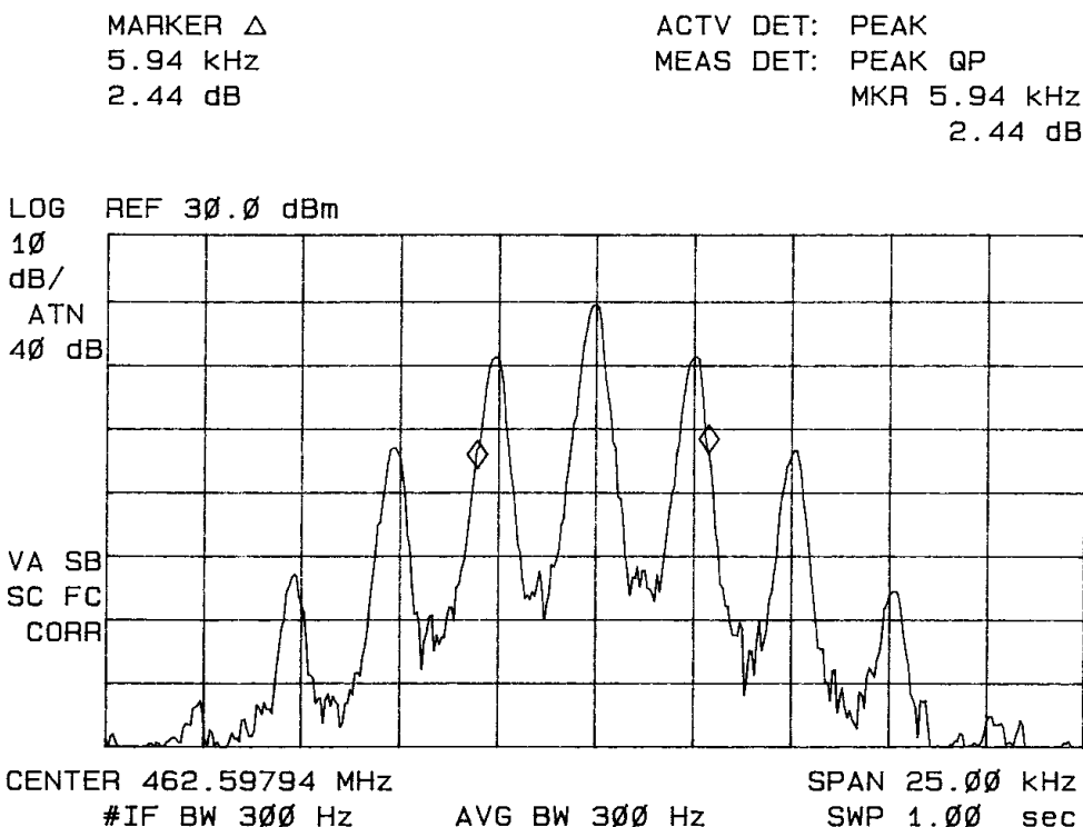
Figure 5: Occupied Band Width, Channel Width 12.5 kHz (1W)
