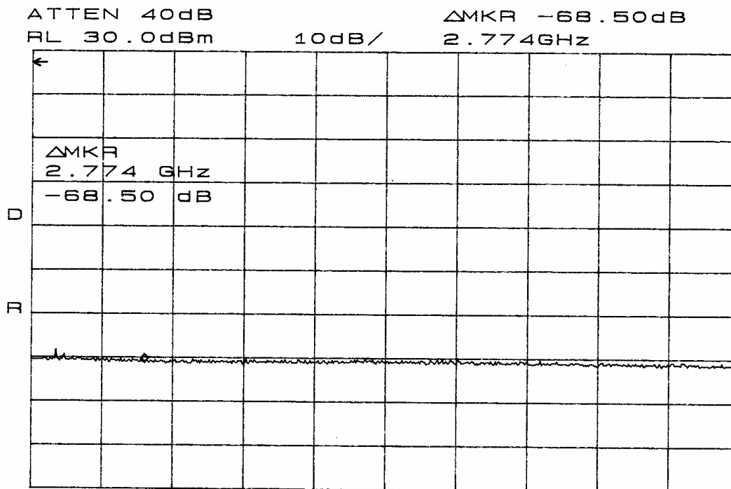
Figure seven Emissions at Antenna Terminal low power.
