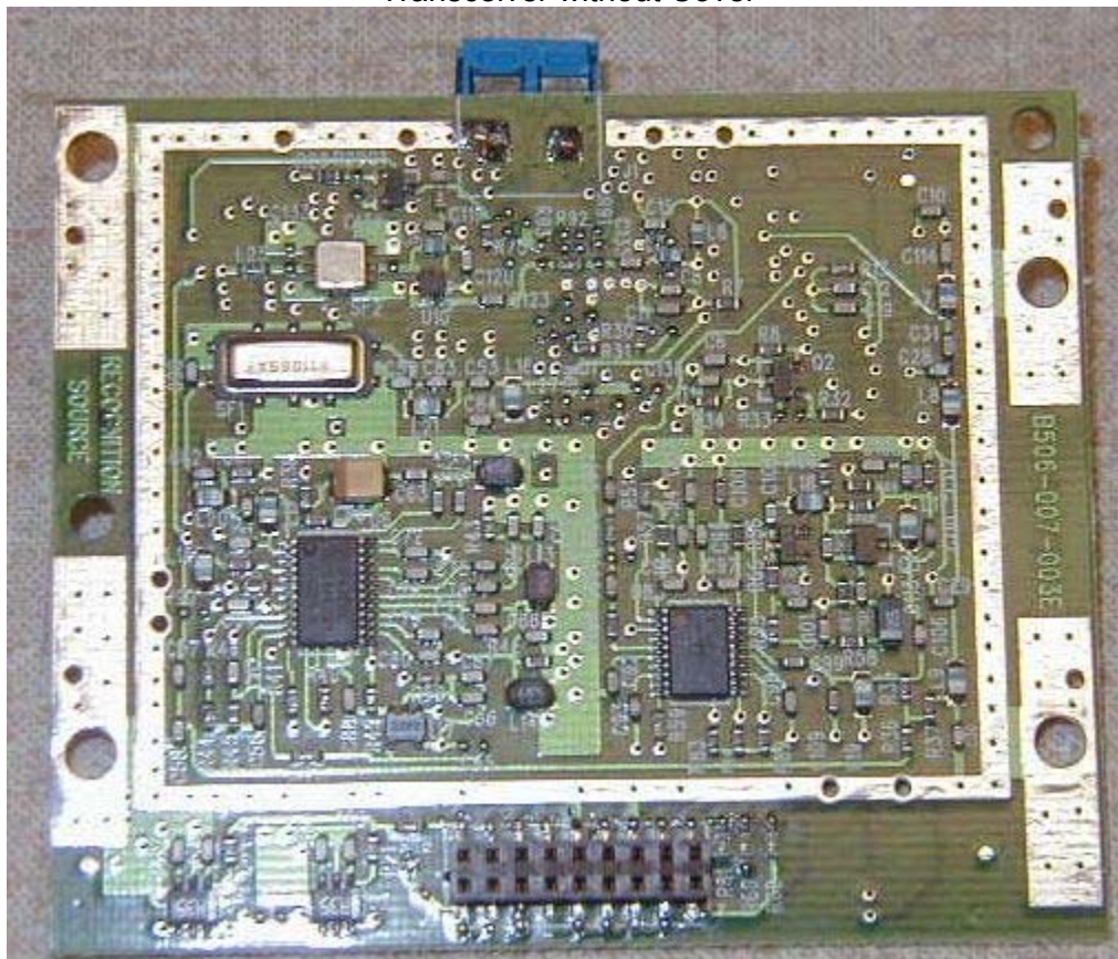
Transceiver without Cover
