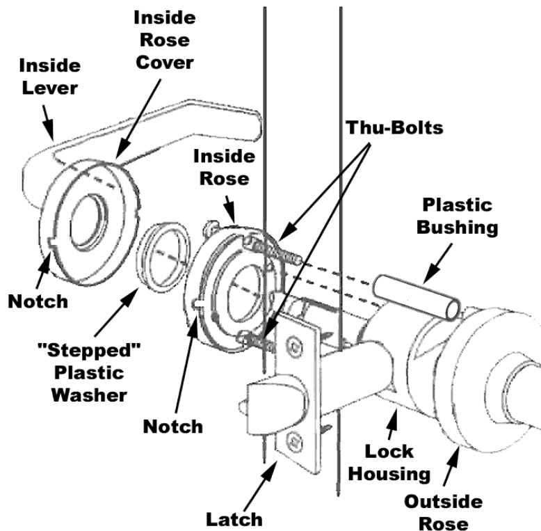
Figure 2-32 – Installing Inside Rose, Thru-Bolts and Cover
