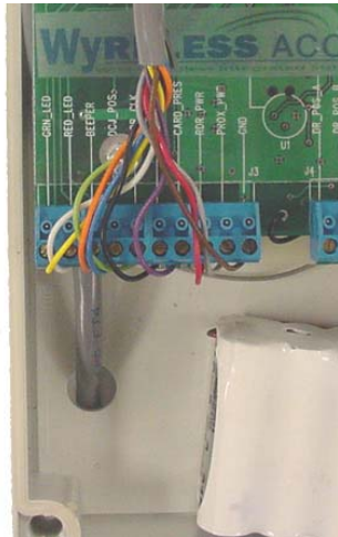
Figure 2-1 – Improper Wire Routing
