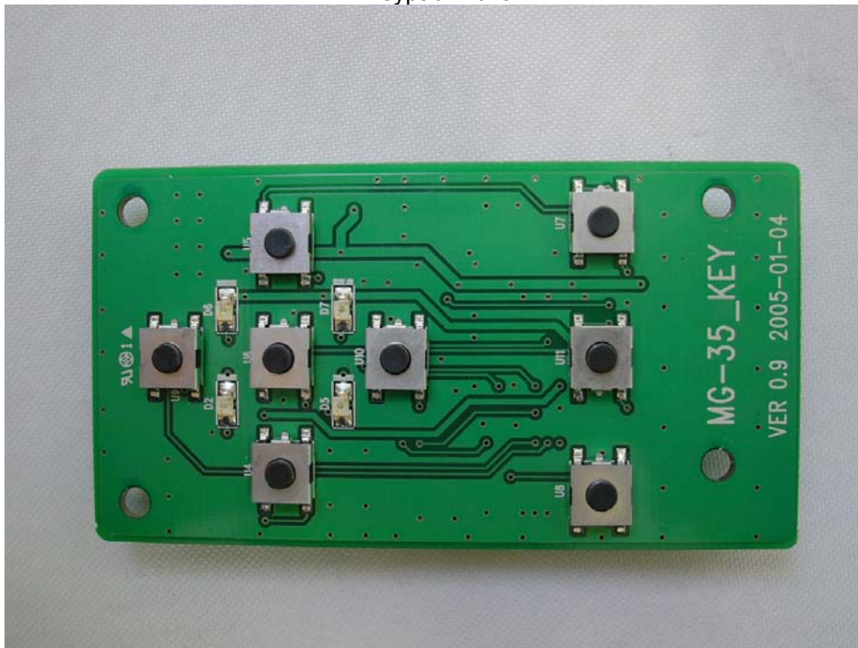
Keypad Rear
