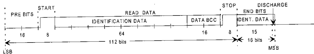
Figure 15: R/W Read Data Format
