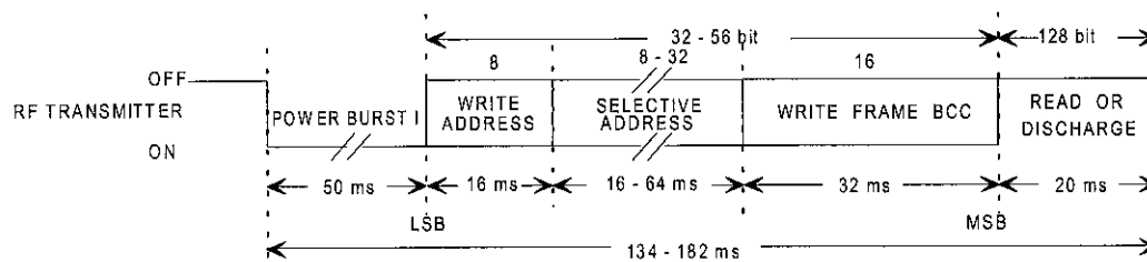
Figure 11: Data Format of the Selective Read Page Function
