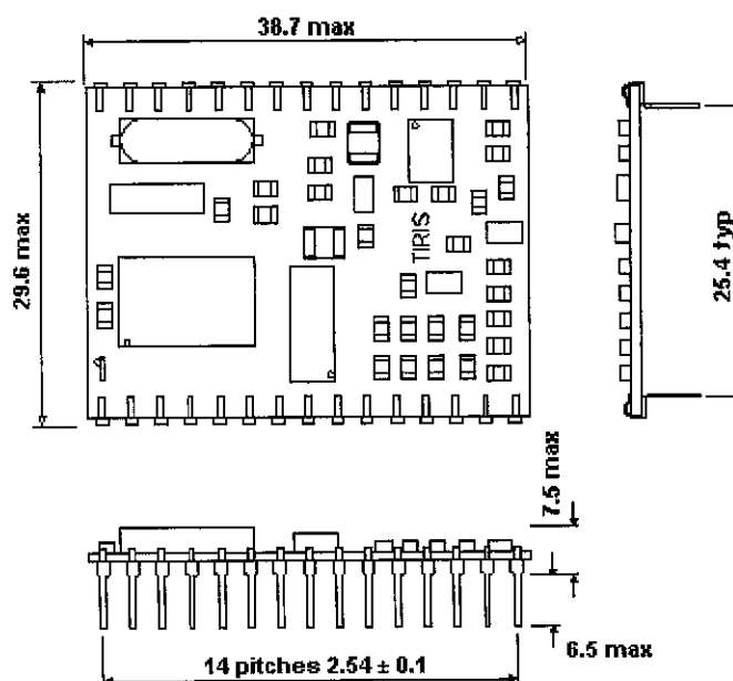
Figure 5: Top, Front and Side View (measurements in mm)
