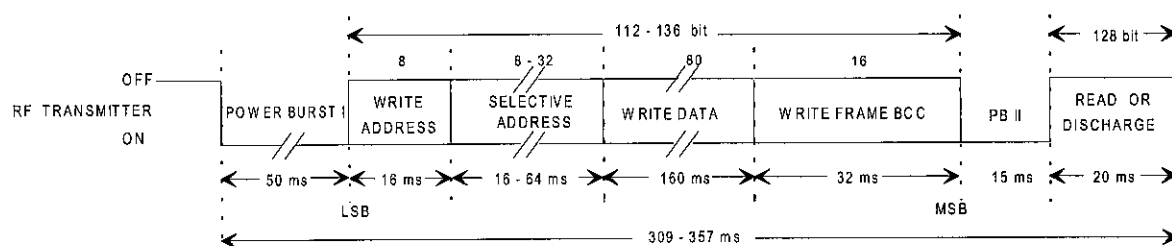
Figure 12: Data Format of the Selective Program Page Function
