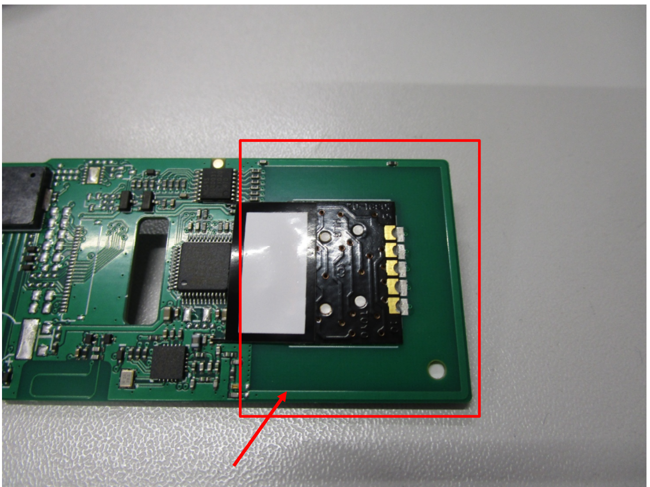
Printed loop antenna
