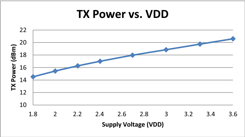
Figure 12. +20 dBm TX Power vs. VDD
