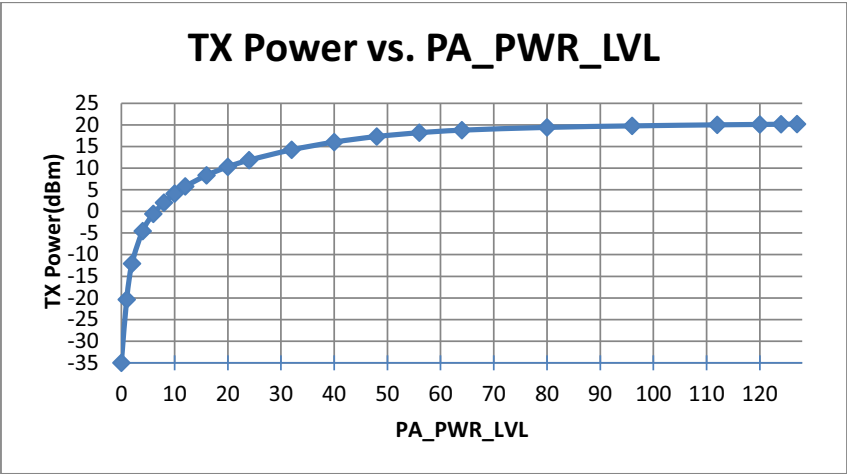
Figure 11. +20 dBm TX Power vs. PA_PWR_LVL
