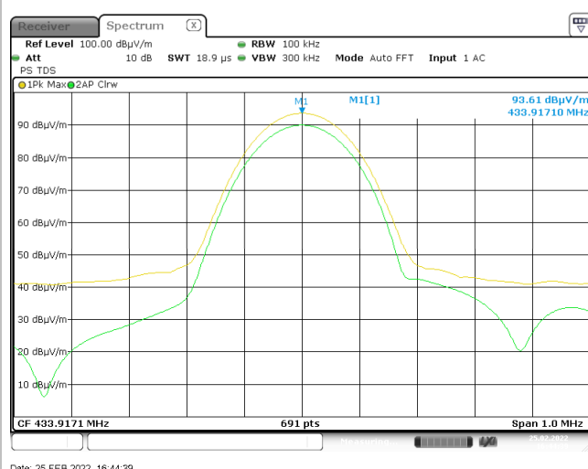
Plot 1 – GFSK modulation
