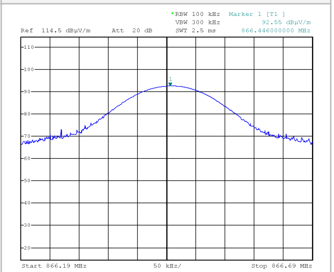
Plot 2 – CH 2
