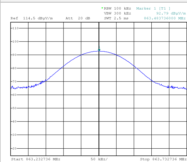
Plot 1 – CH 1
