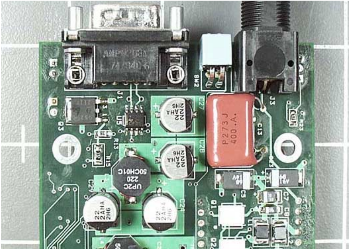
PCB 1 Bottom Closeup 2
