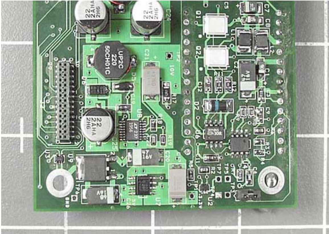
PCB 1 Bottom Closeup 1
