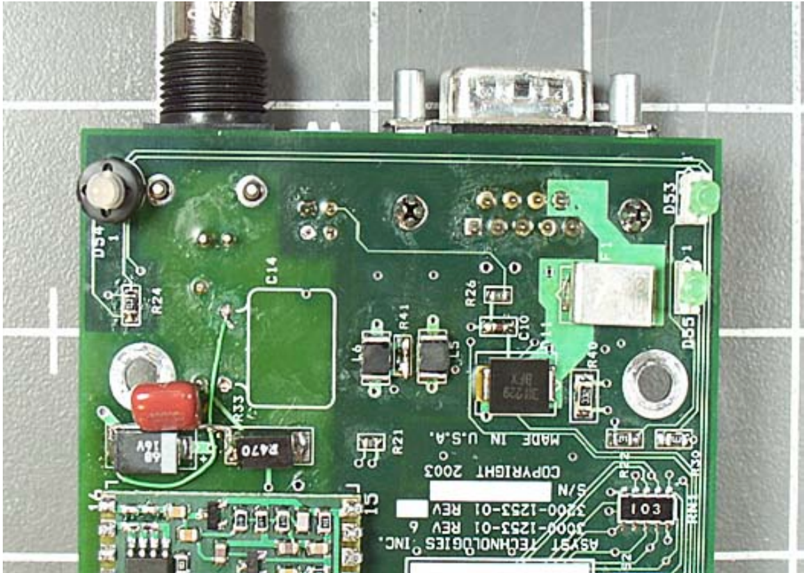
PCB Top Closeup 2
