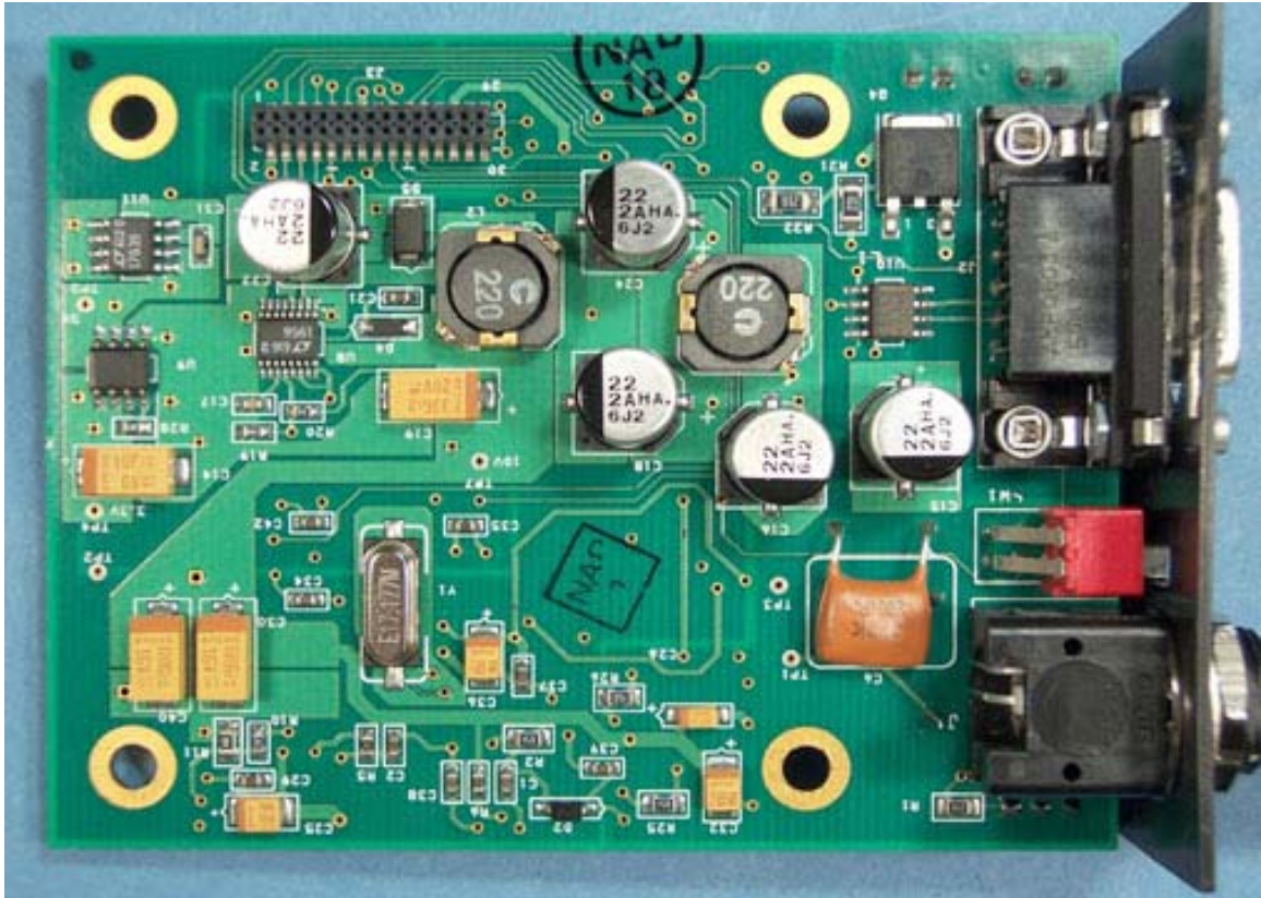
Top Board Bottom Side
