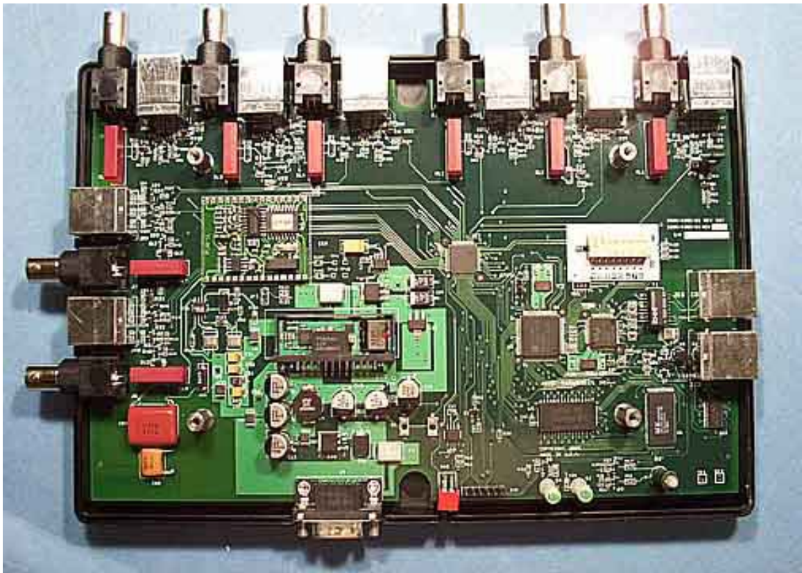
Top with Chassis cover removed
