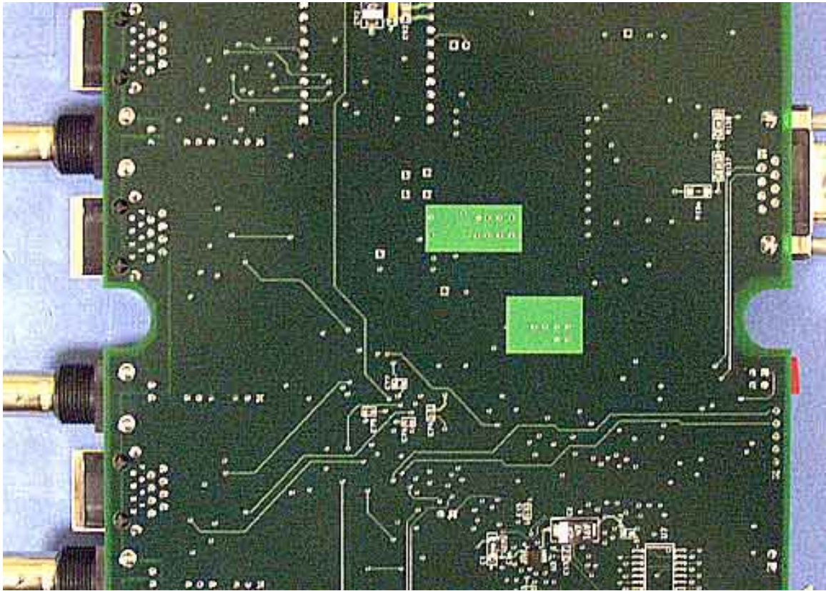
Bottom of Board Center
