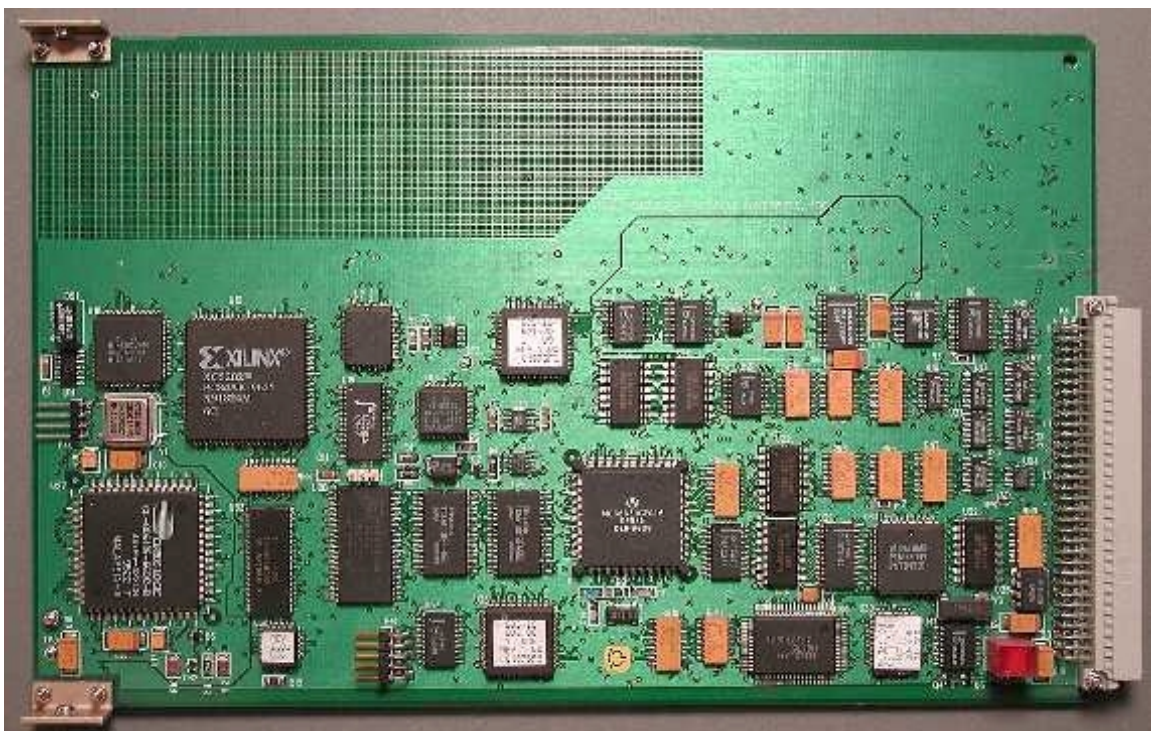
This is the top side of the Input/Output (IOP) board.
