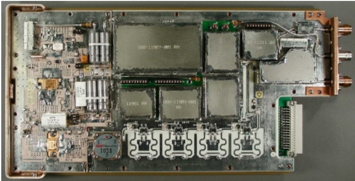
This is the top side of the RF board assembly. There is a cover over this board when it is put in the assembly.
