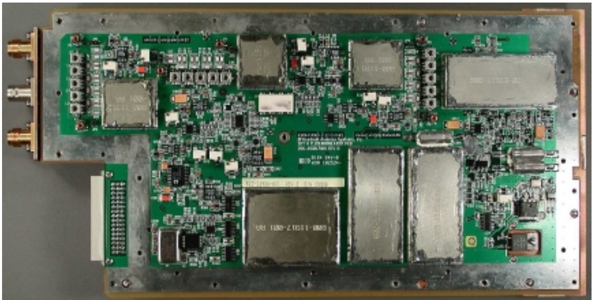
This is the bottom side of the RF board assembly. There is a cover over this board when it is put in the assembly.
