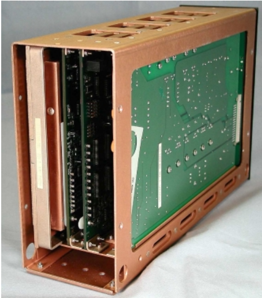
This is the back of the unit with its cover off. From Left to right: RF assembly, Surveillance board (computer board) , Input Output board, Power Supply.
