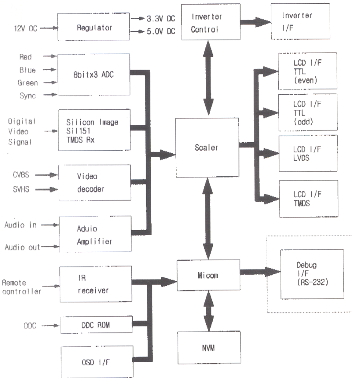
3-3 Block Diagram
