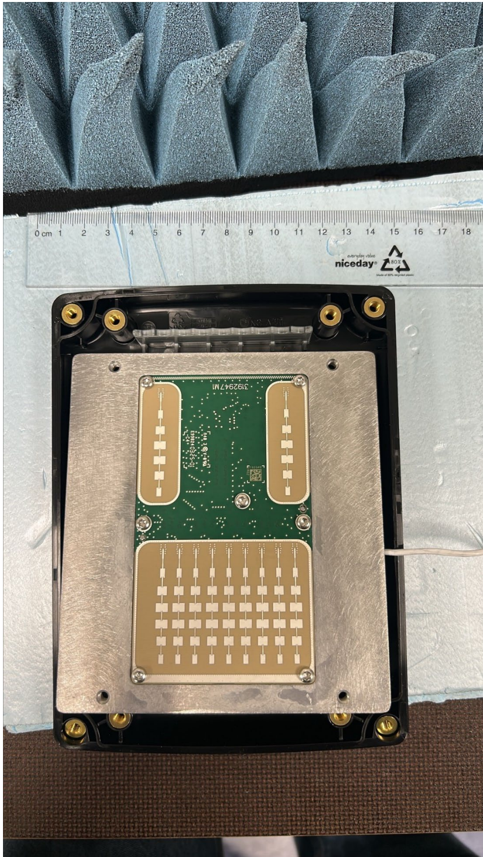
Figure 7: RF PCB front
