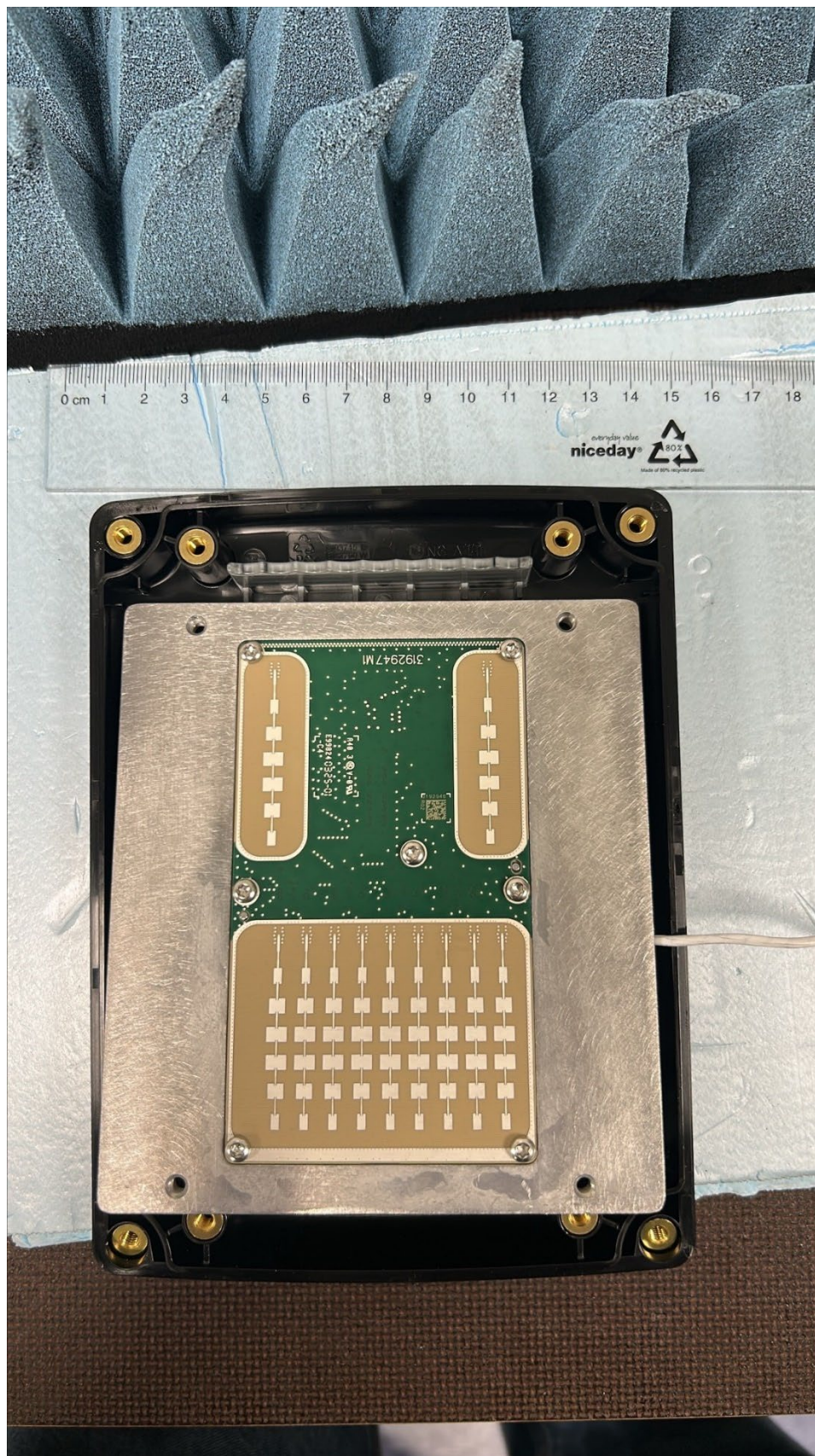
Figure 7: RF PCB front
