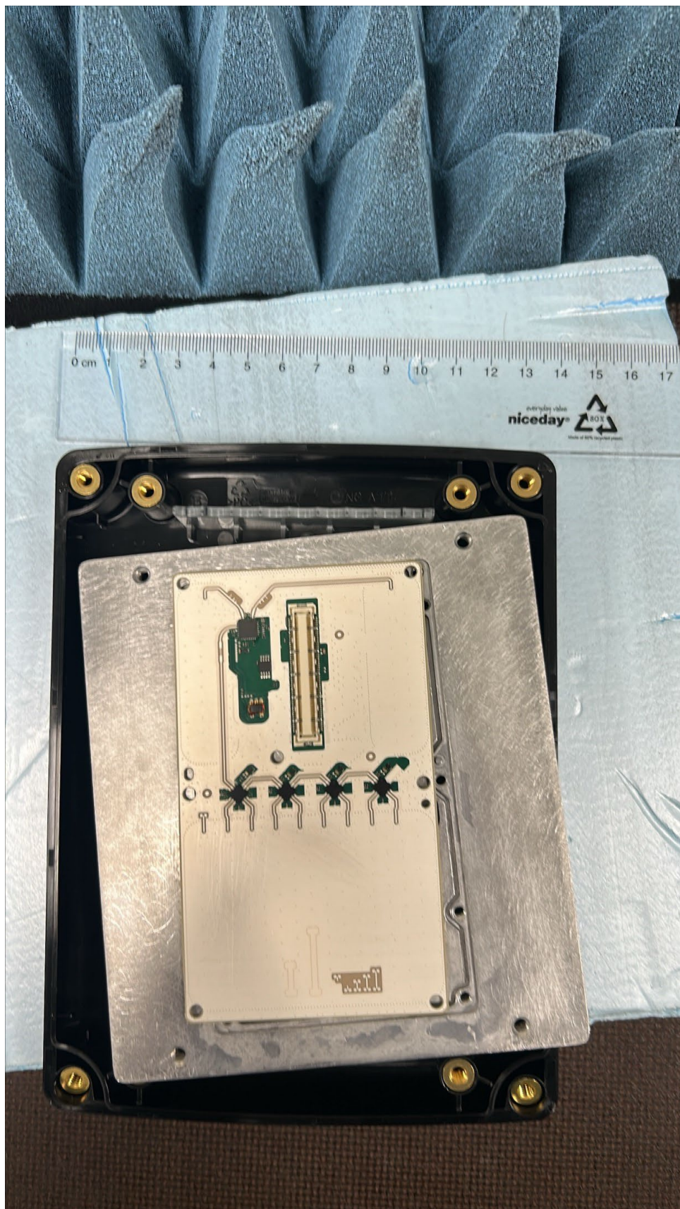
Figure 8: RF PCB back
