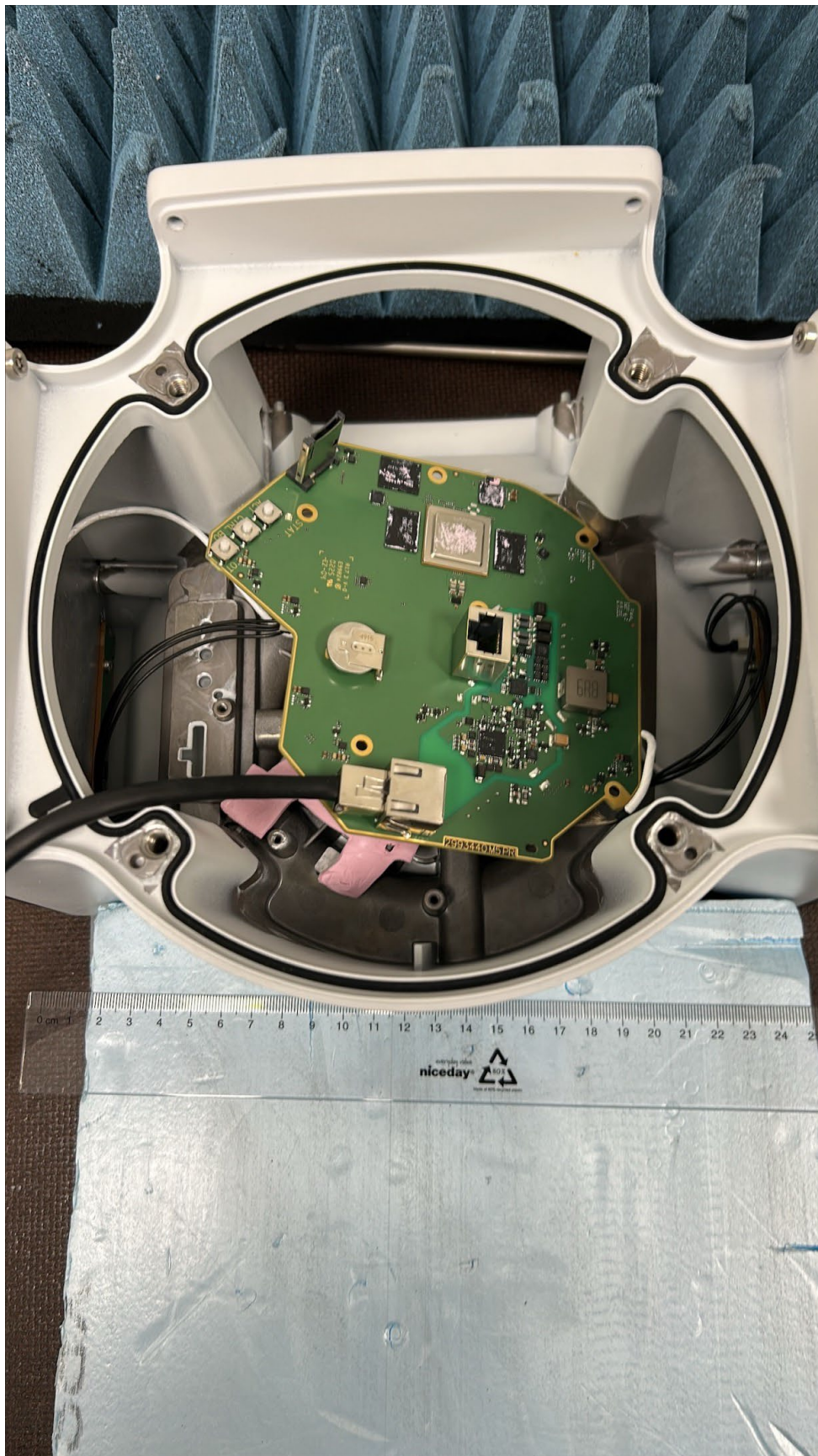
Figure 3: Main PCB back
