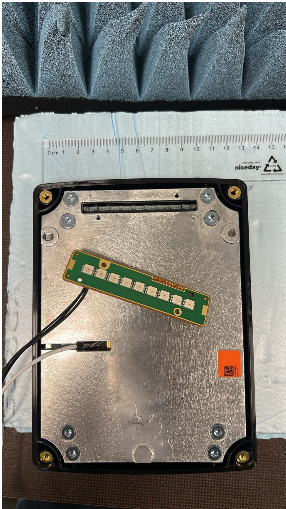
Figure 5: RF module back, flipped LED PCB
