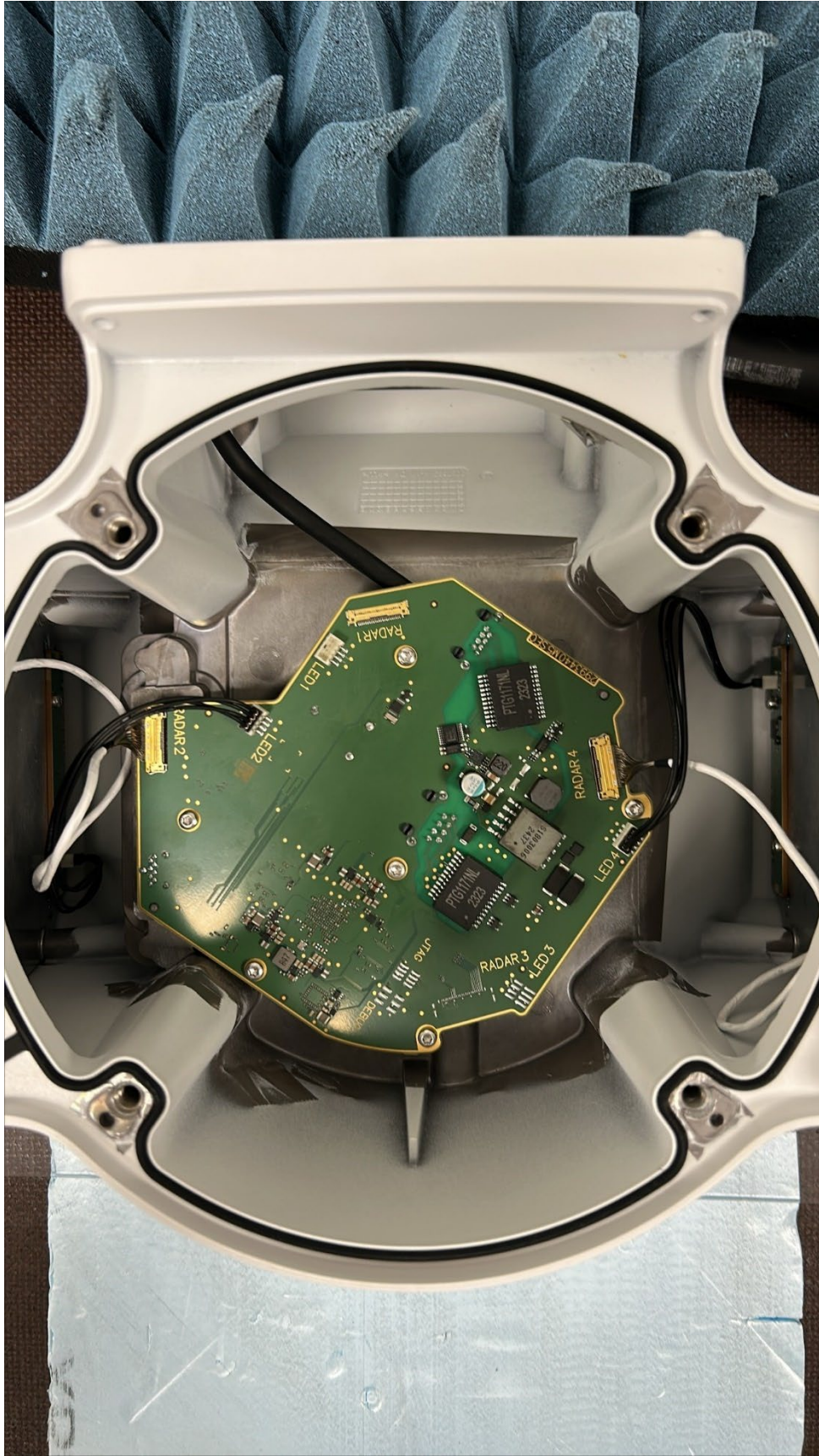
Figure 2: Main PCB front
