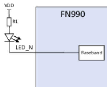
Figure 16: Recommended LED Connection
