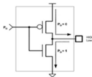
Figure 18: GPIO Output Pin Equivalent Circuit
