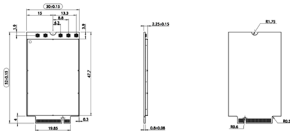
Figure 22: FN990 Family Module Mechanical Dimensions
