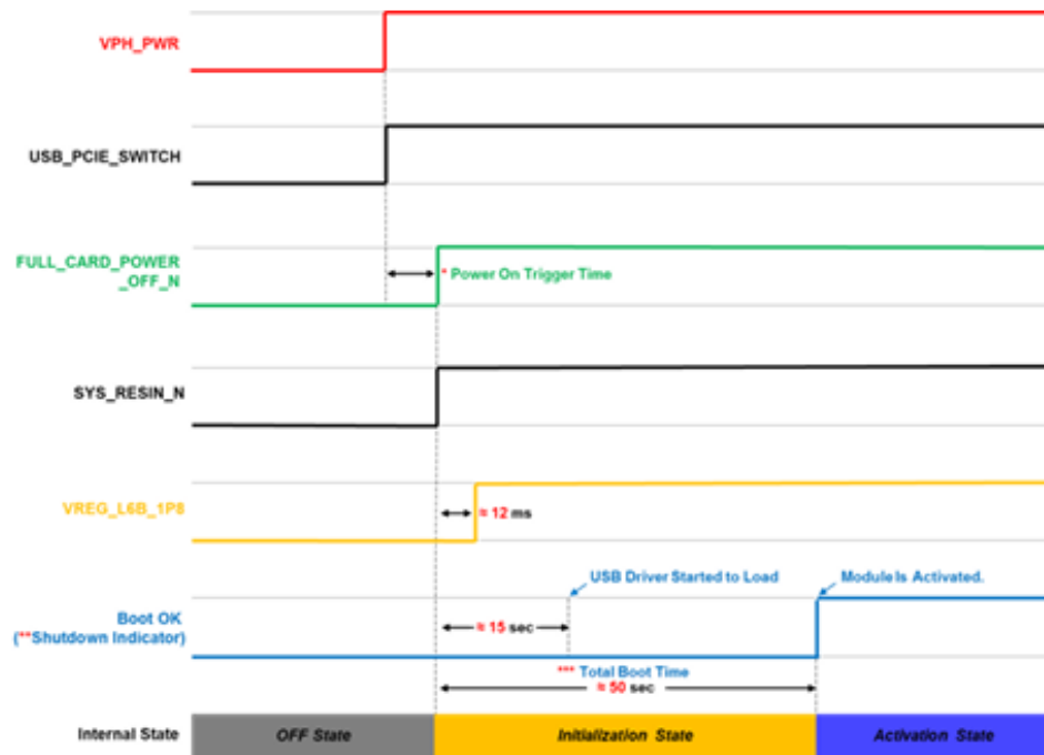
Figure 3: FN990 Family Power ON Sequence - USB mode (USB_PCIE_SWITCH: High, Default)
