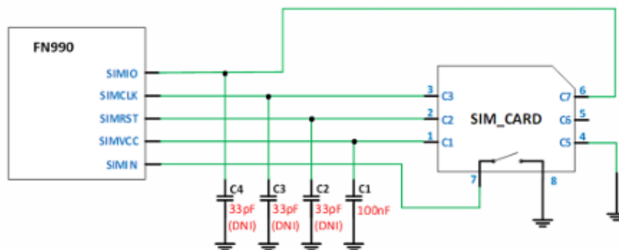
Figure 14: SIM Schematic Example
