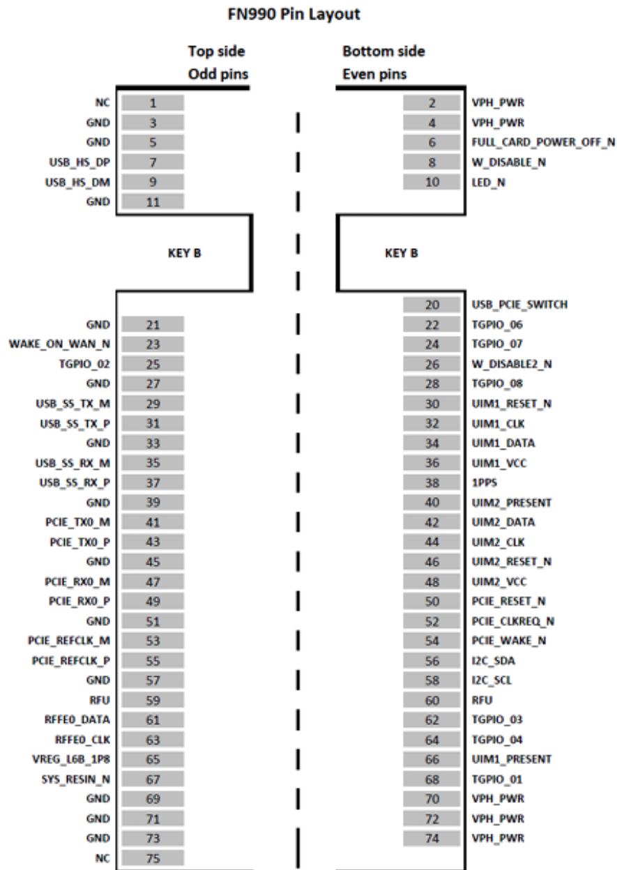
Figure 2: FN990 Family Pinout
