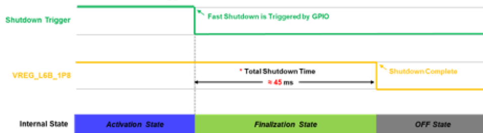
Figure 7: Fast Shutdown by GPIO
