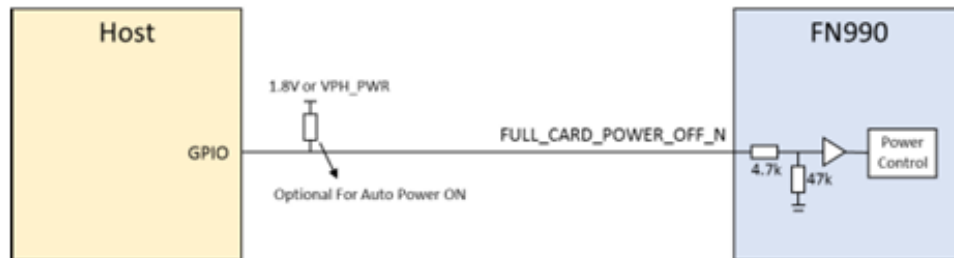
Figure 5: Example Circuit for ON/OFF by FULL_CARD_POWER_OFF_N
