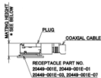
Figure 20: MHF-4 RF connector
