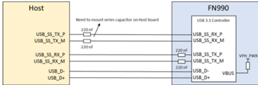
Figure 13: Connection for USB Interface
