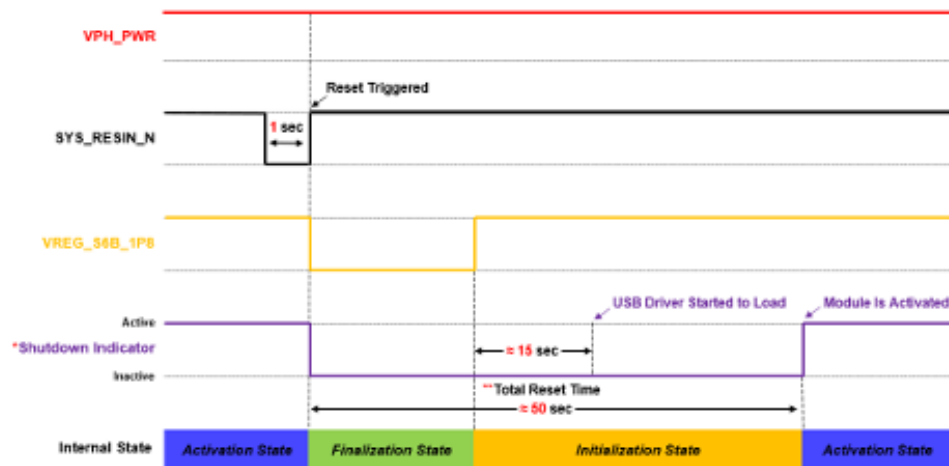
Figure 9: Unconditional Hardware Reset by SYS_RESIN_N
