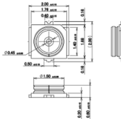
Figure 20: MHF-4 RF connector
