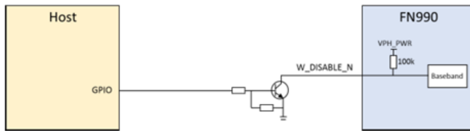
Figure 15: Example Circuit for WLAN/GNSS Disable Function
