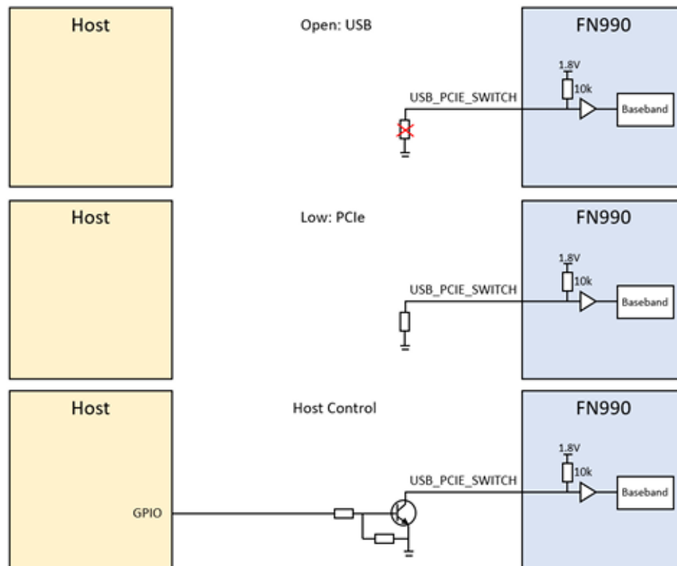
Figure 11: Example Circuit for HOST Interface Switch Function
