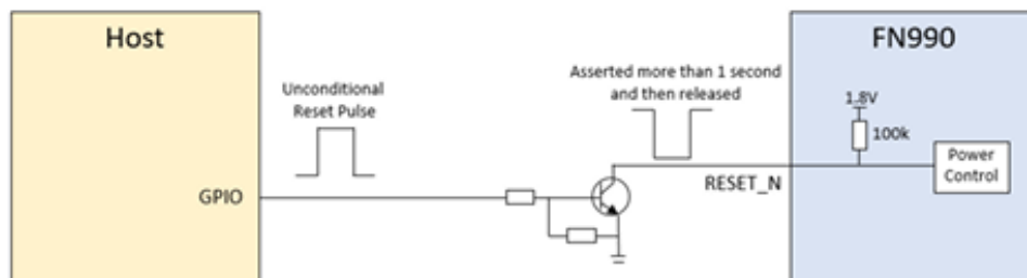
Figure 10: Example Circuit for RESET by SYSTEM_RESET_N
