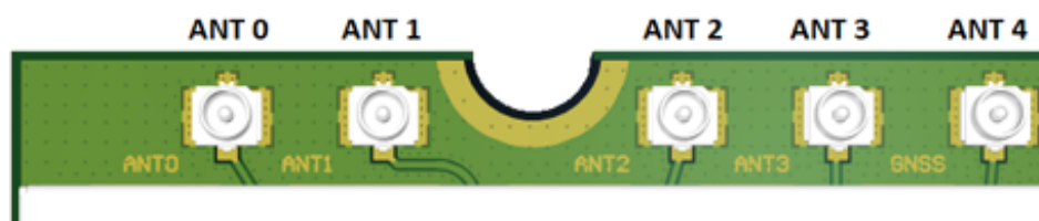
Figure 19: Antenna Configuration
