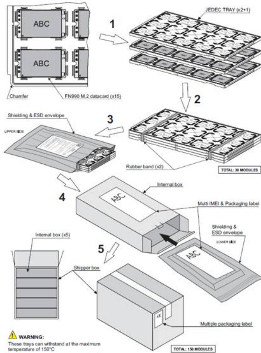
Figure 23: Tray Packaging
