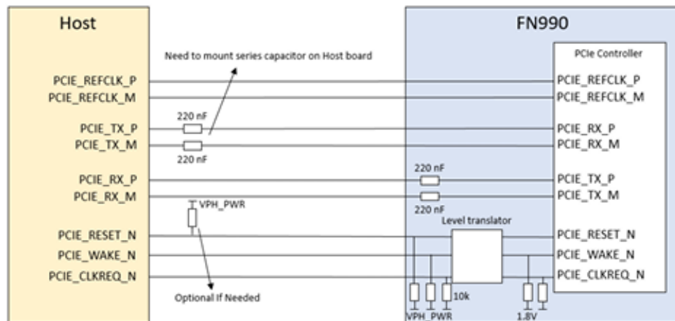
Figure 12: Connection for PCIe Interface
