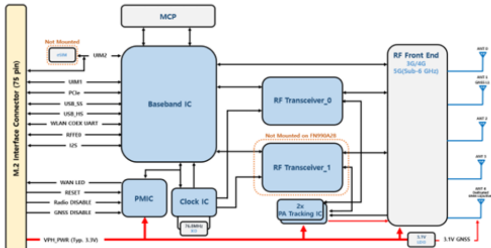
Figure 1: FN990 Family Block Diagram
