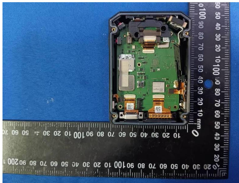
Internal View of EUT-4
