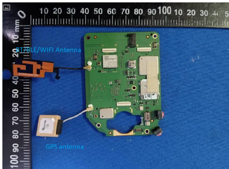
Internal View of EUT-4
