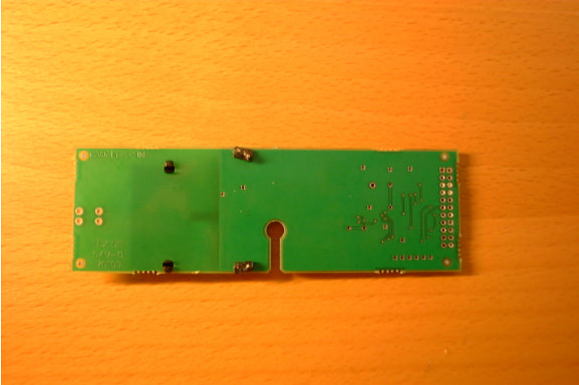
Bottom of Alps Bluetooth implementation board used by Axis
