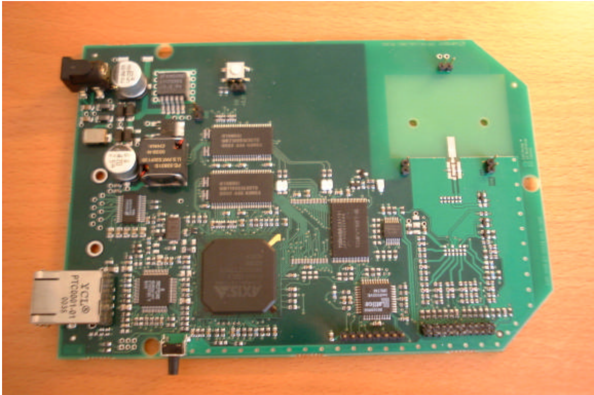
Top view main board with Alps board removed
