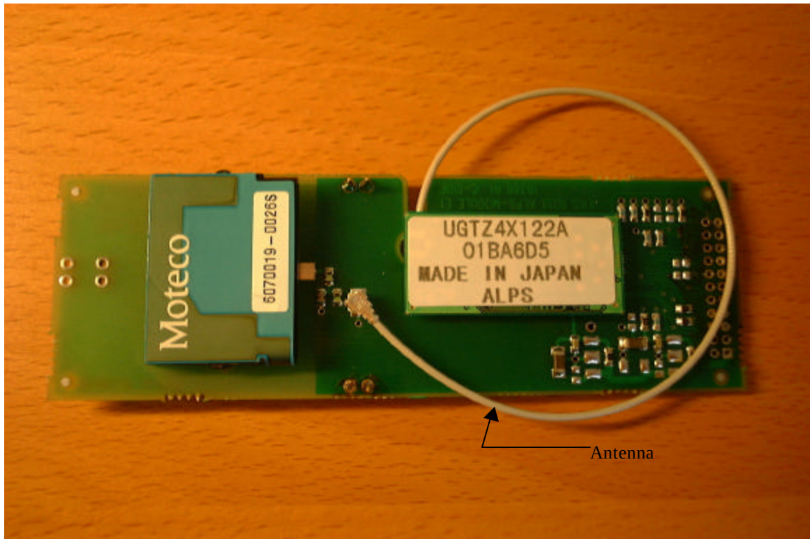
Top of Alps Bluetooth Implementation Board showing antenna.
