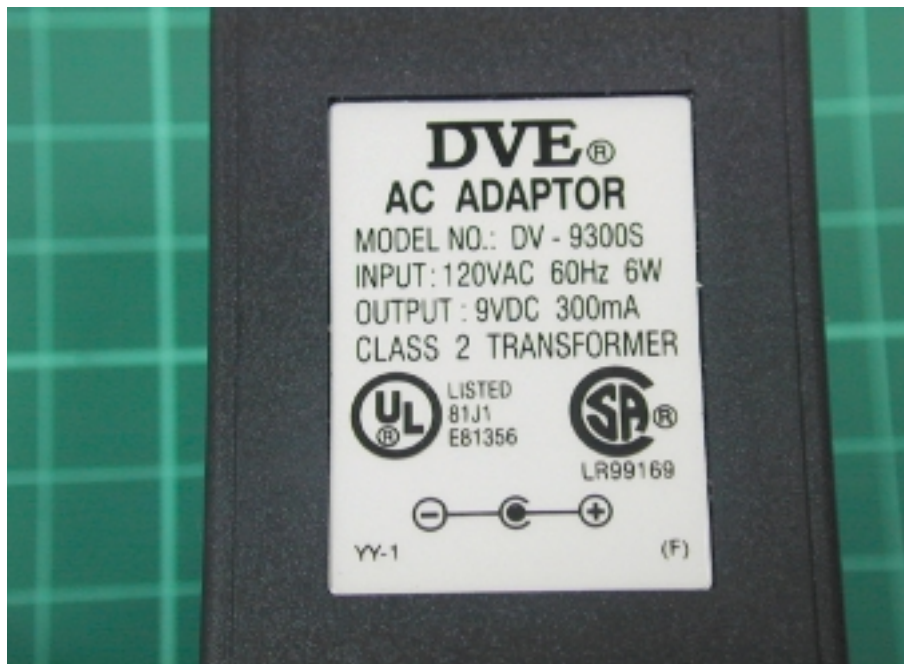
Photo 3: Photo of Adapter
