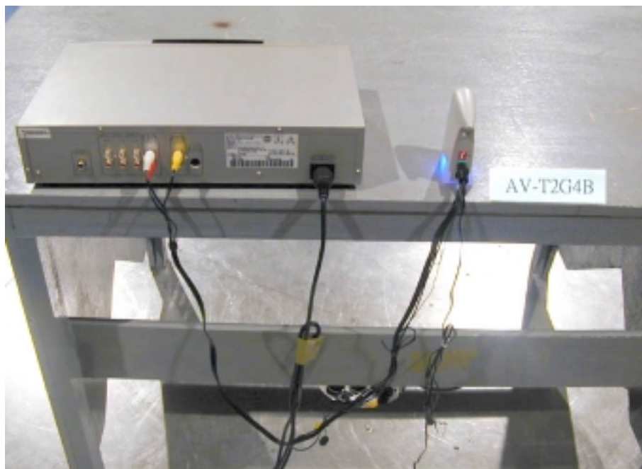
Photo 2: Radiated Emission Test Set-up (rear)
