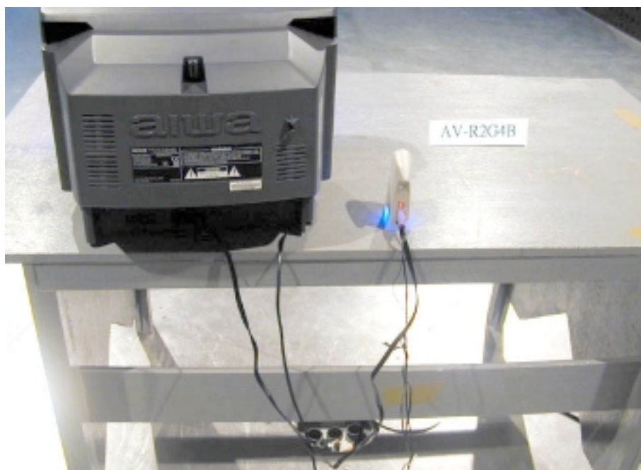
Photo 2: Spurious Emission Test Set-up (rear)
