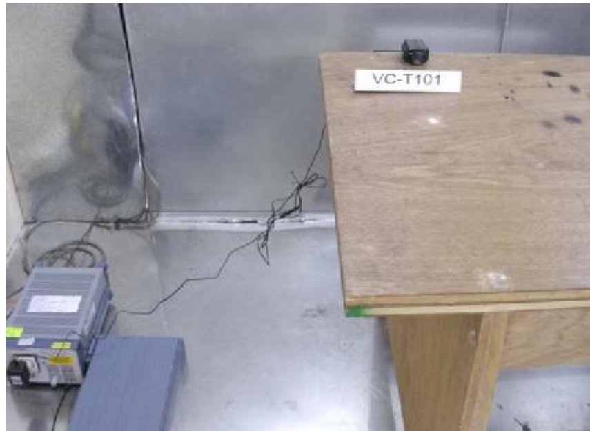
Photo 2: Conducted Test Set-up photo (rear)
