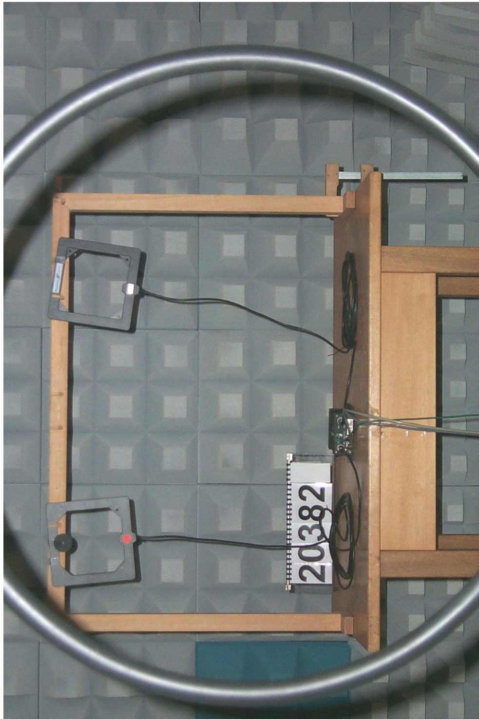
20382_d.jpg OISL 77LA04/2-SER test set-up preliminary emission test (9 kHz to 30 MHz)
