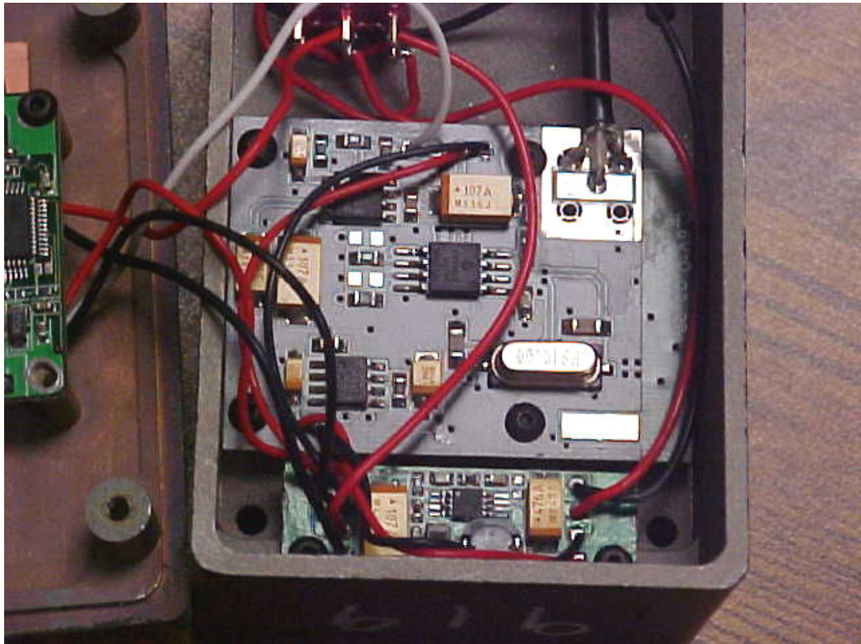
Transmitter Board – Component View
