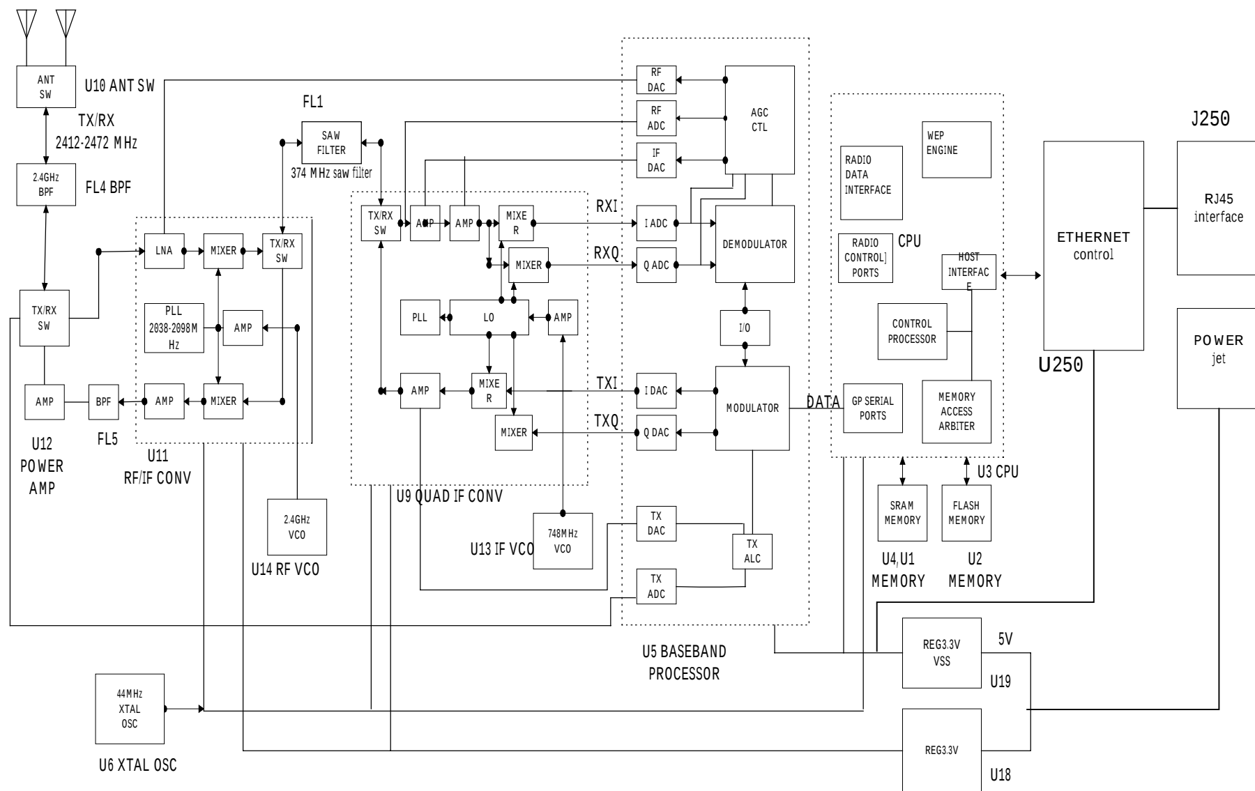
WX-1500 Block Diagram
