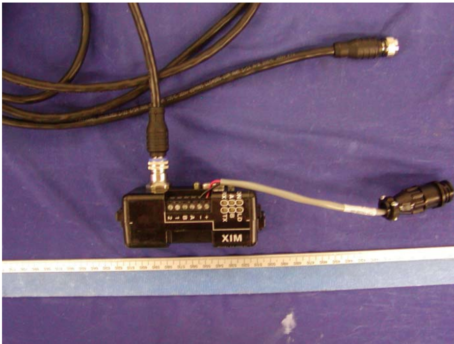
XIM Interface Module and Cable
