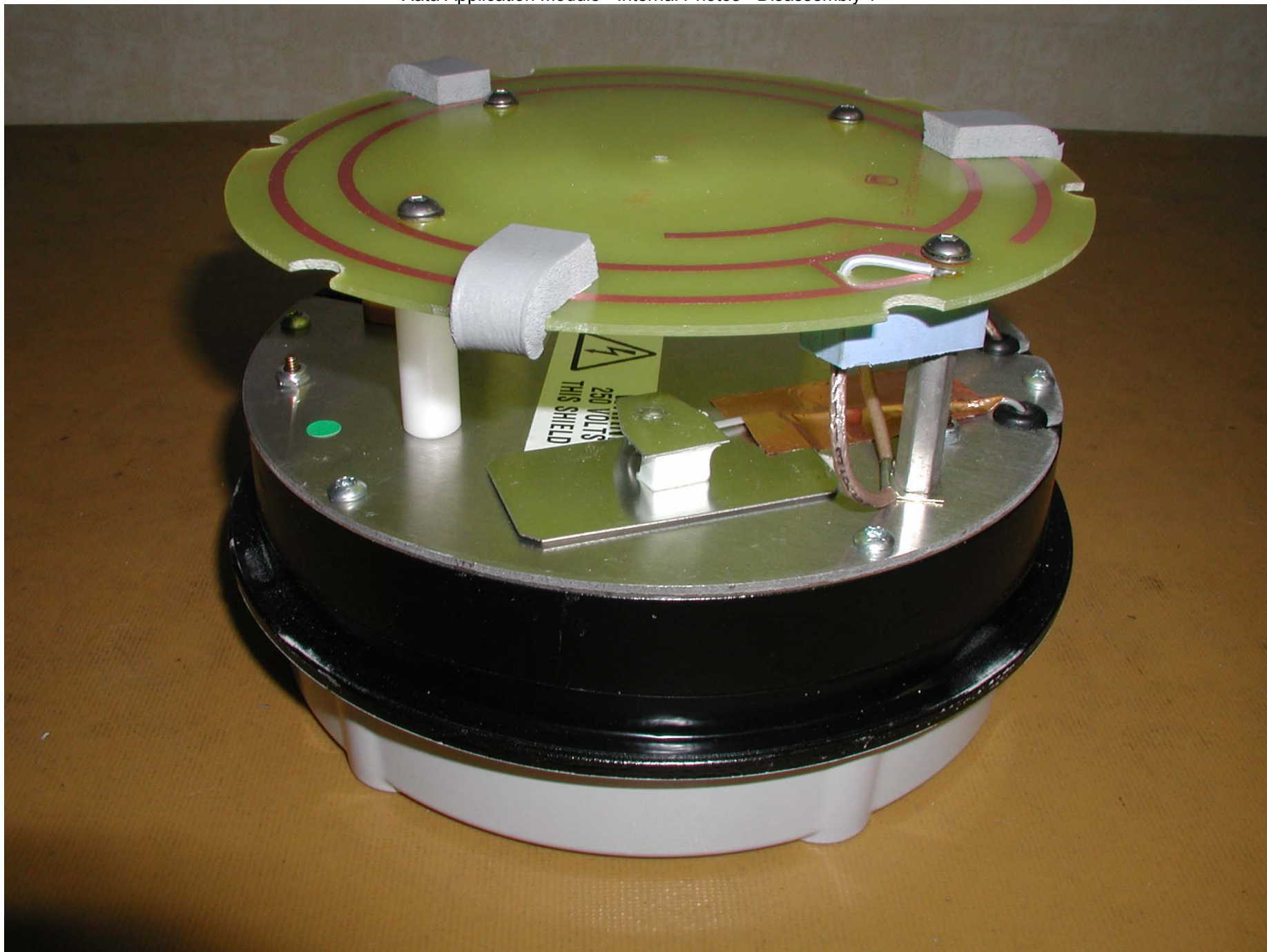
Xata Application Module - Internal Photos - Disassembly 1
