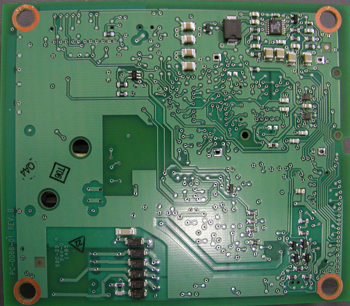
Xata Application Module - Internal Photos - Peripheral Board Bottom
