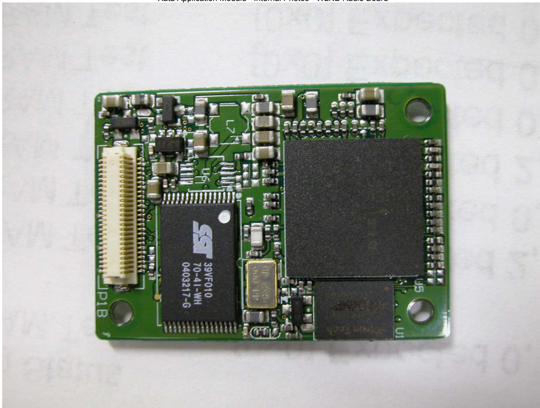
Xata Application Module - Internal Photos - WLNb Radio Board
