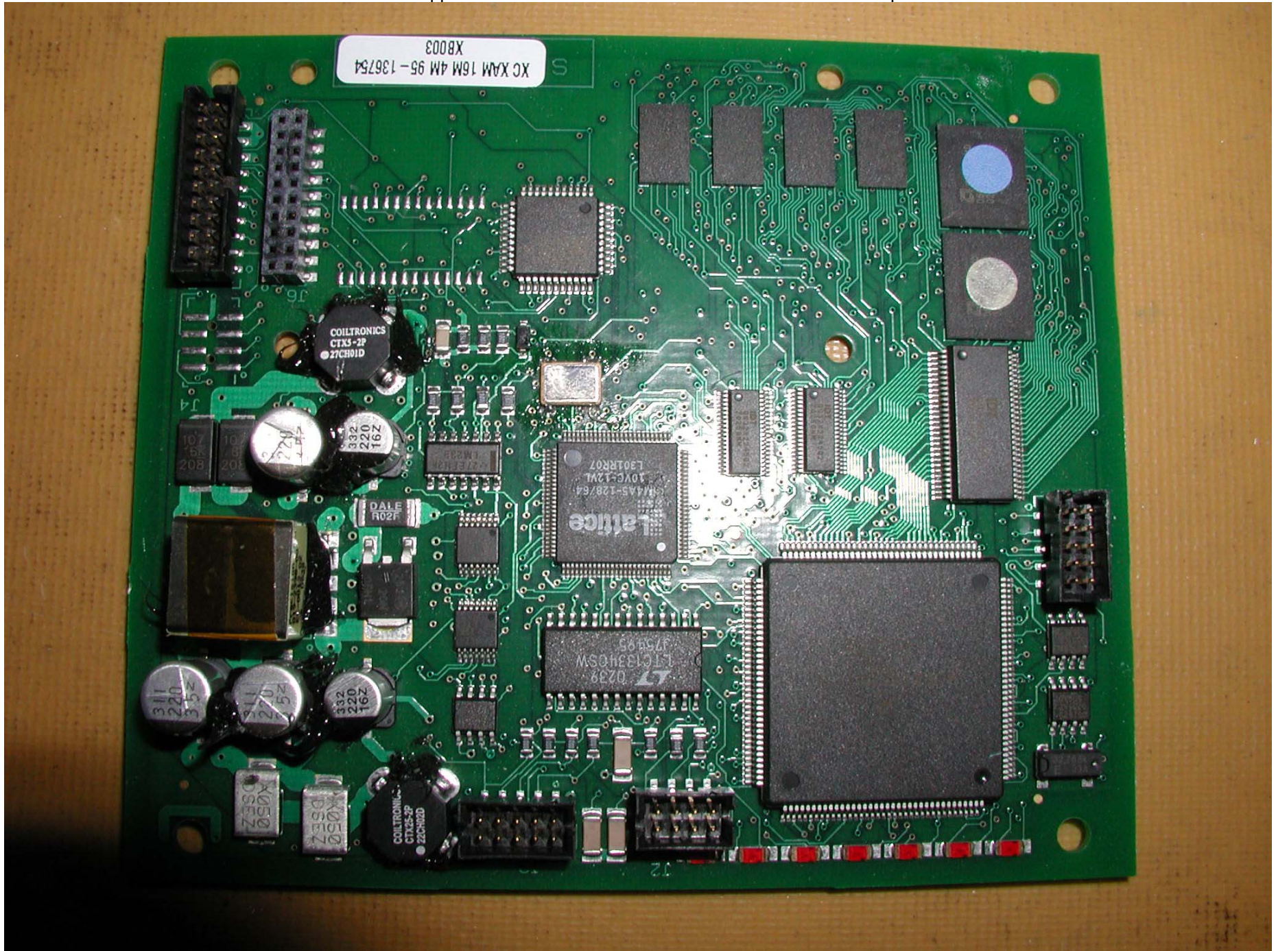
Xata Application Module - Internal Photos - Processor Board Top
