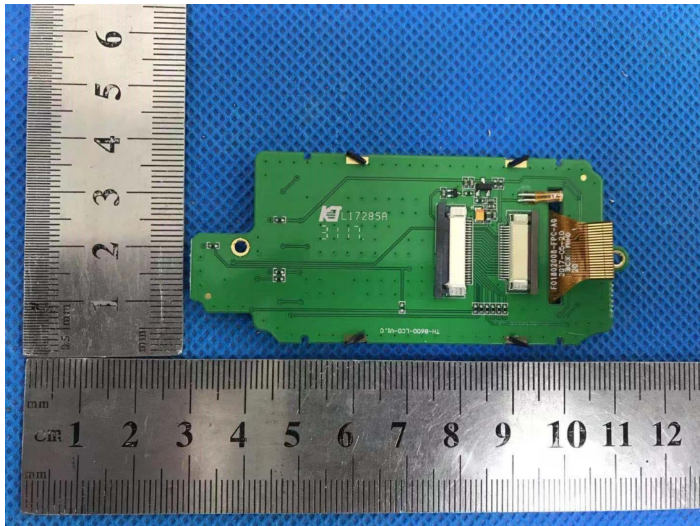
INTERNAL VIEW-5 OF EUT-2
