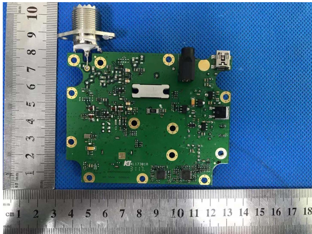
INTERNAL VIEW-4 OF EUT-1
