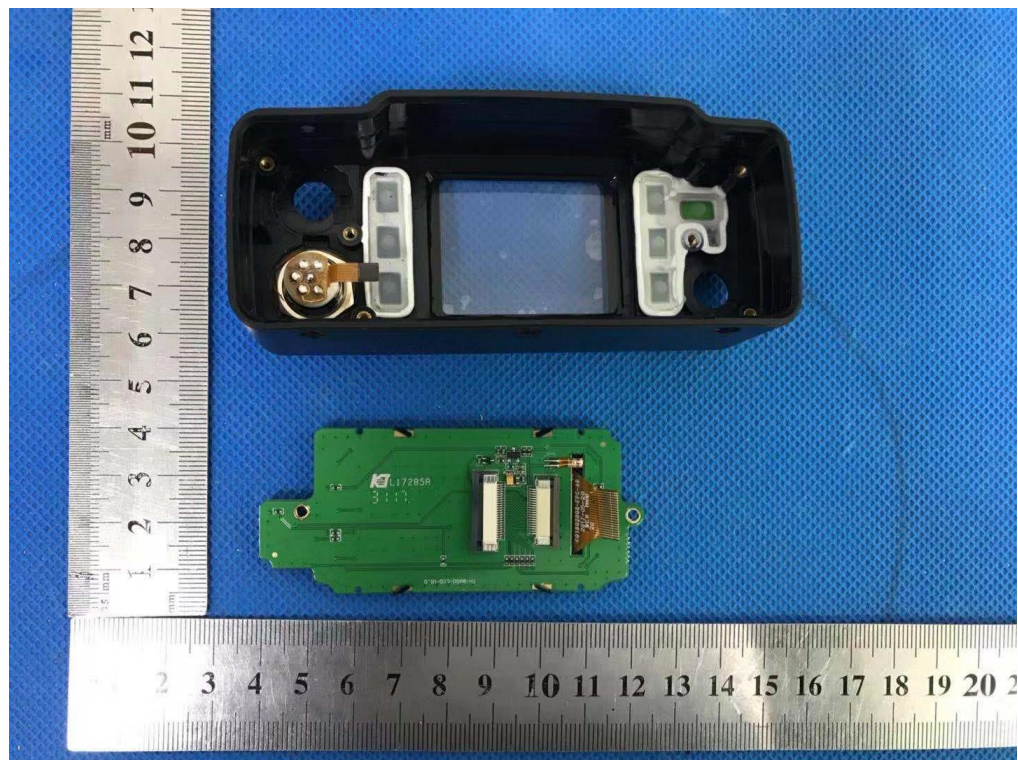
INTERNAL VIEW-1 OF EUT-2
