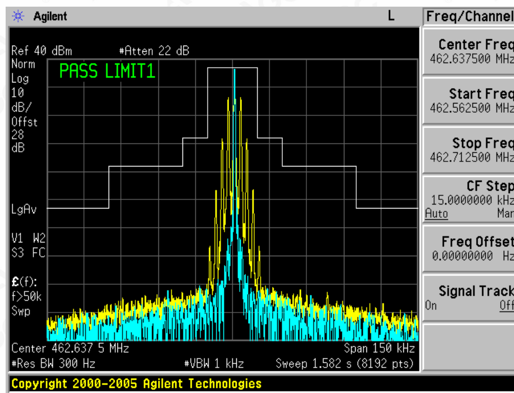
The Worst Emission Mask for channel 4 -5W-12.5K
