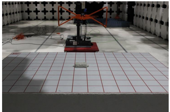
Radiated Emissions Rear (Below 1 GHz)
