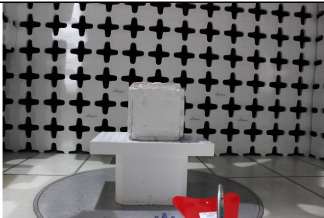
Radiated Emissions Front (Above 1 GHz)
