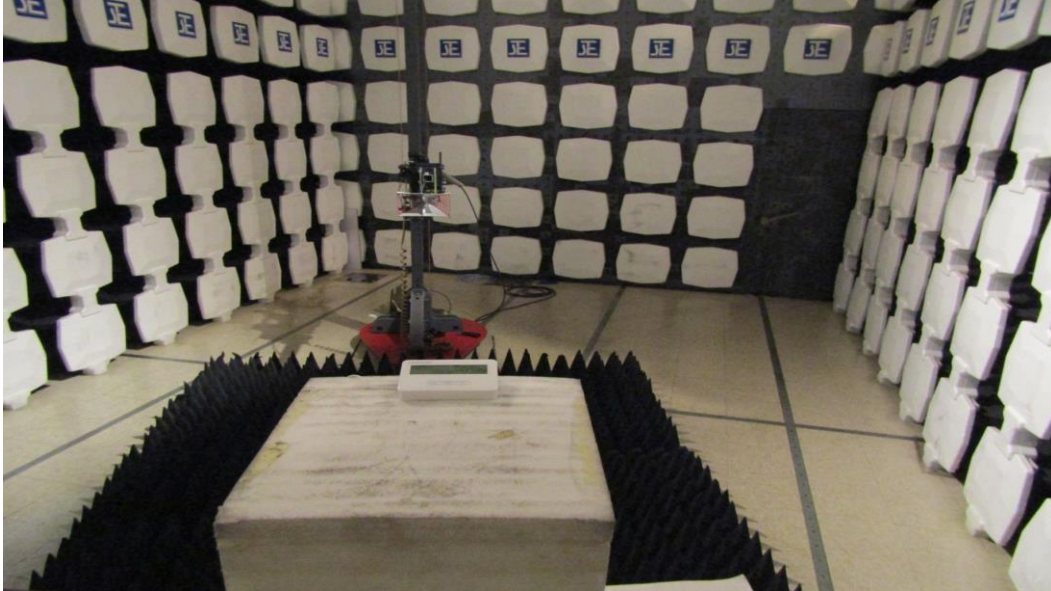
Measurement of Radiated Emission Test Set Up (Above 1000MHz)
