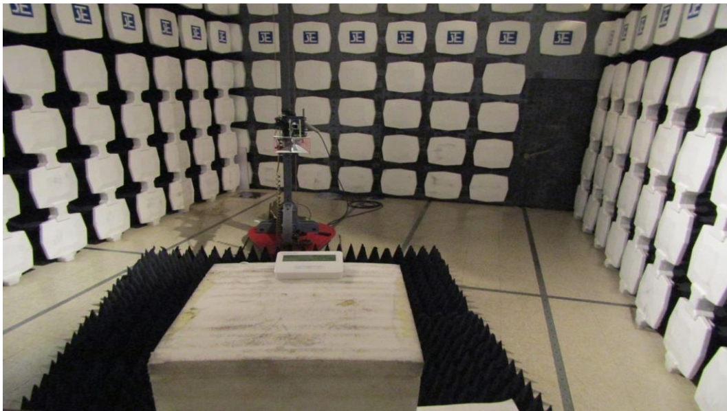
Measurement of Radiated Emission Test Set Up (Above 1000MHz)
