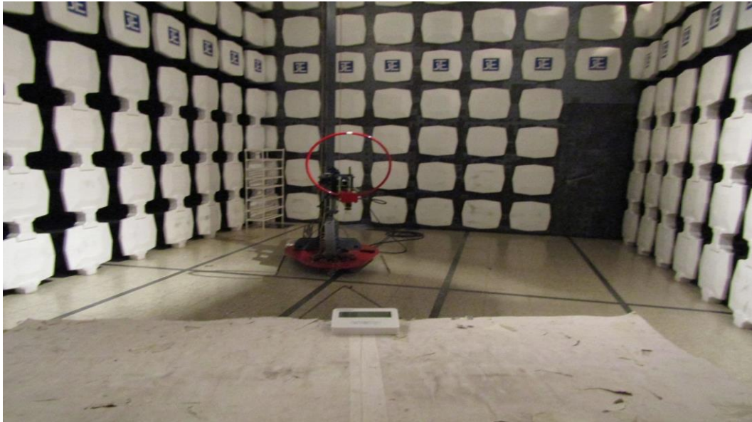
Measurement of Radiated Emission Test Set Up (9kHz to 30MHz)
