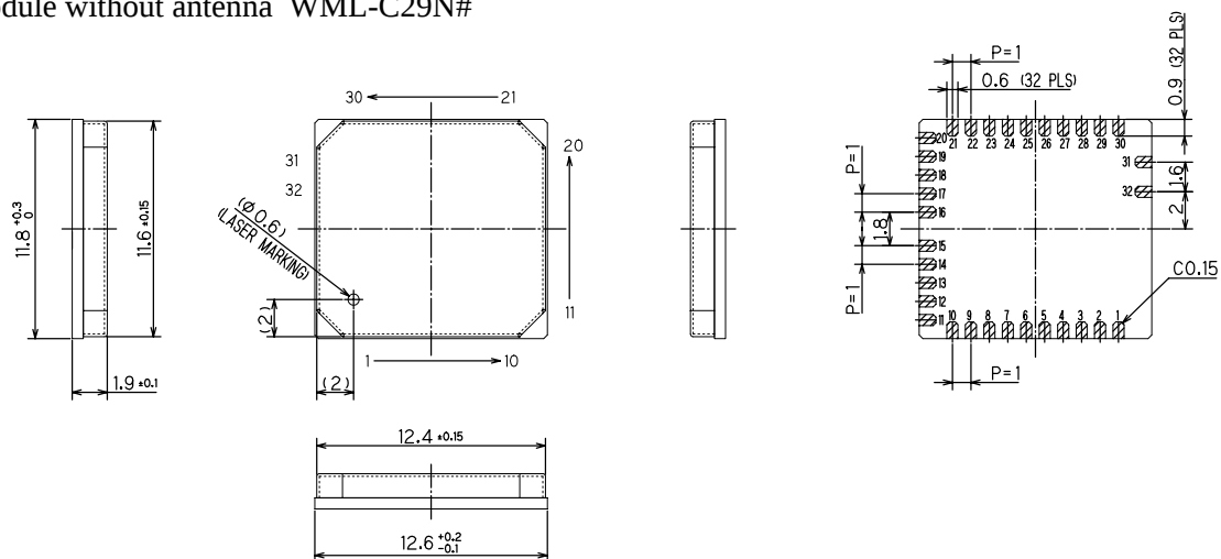
Module without antenna WML-C29N#
