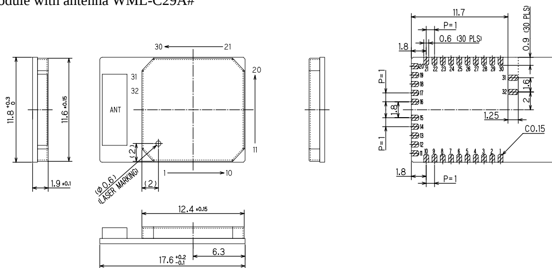
Module with antenna WML-C29A#
