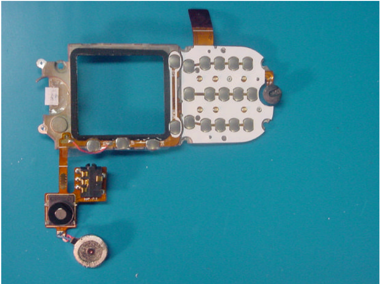
PHOTOGRAPH 7: KEYBOARD FRONT
