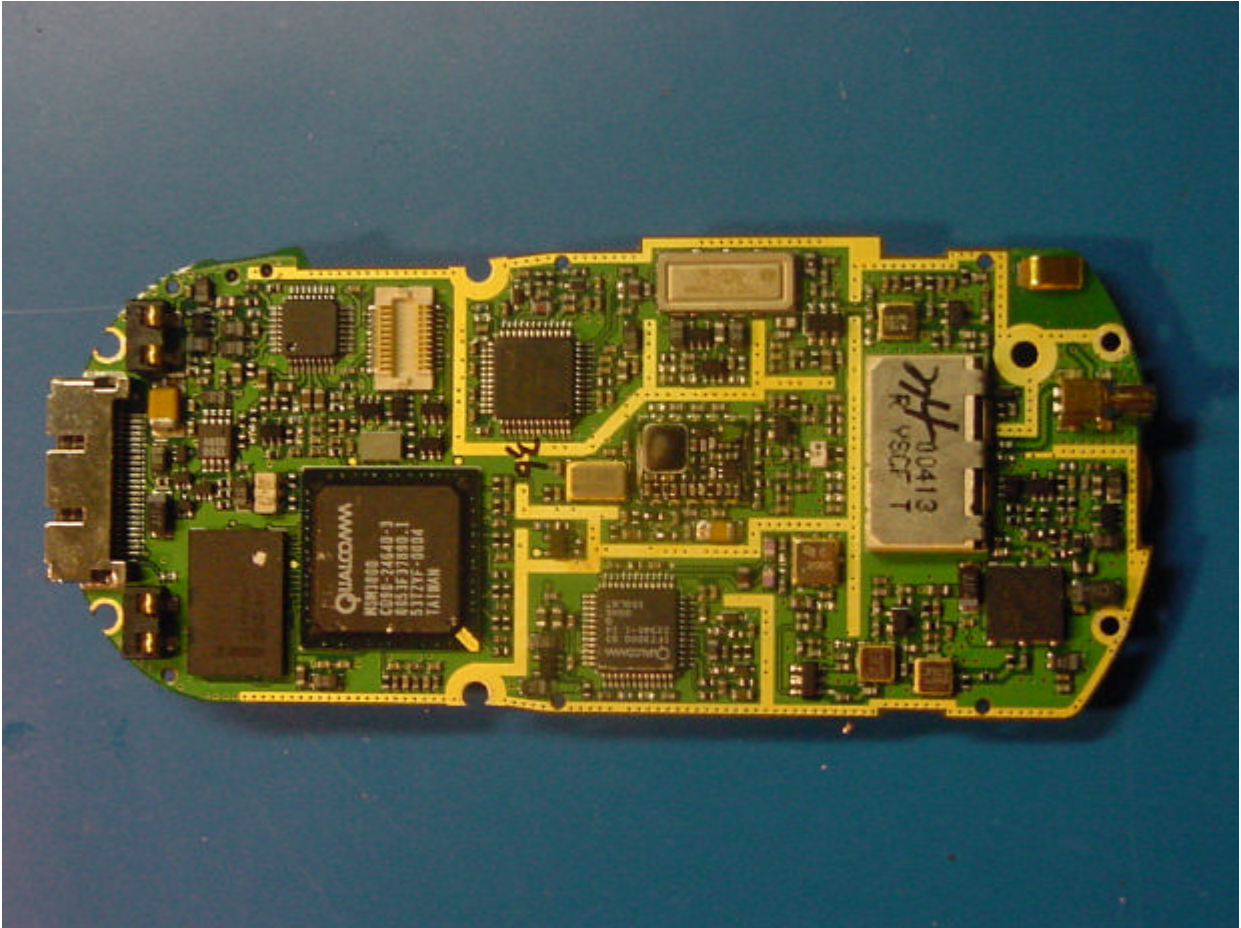
PHOTOGRAPH 12: MAIN BOARD REAR WITHOUT SHIELDS
