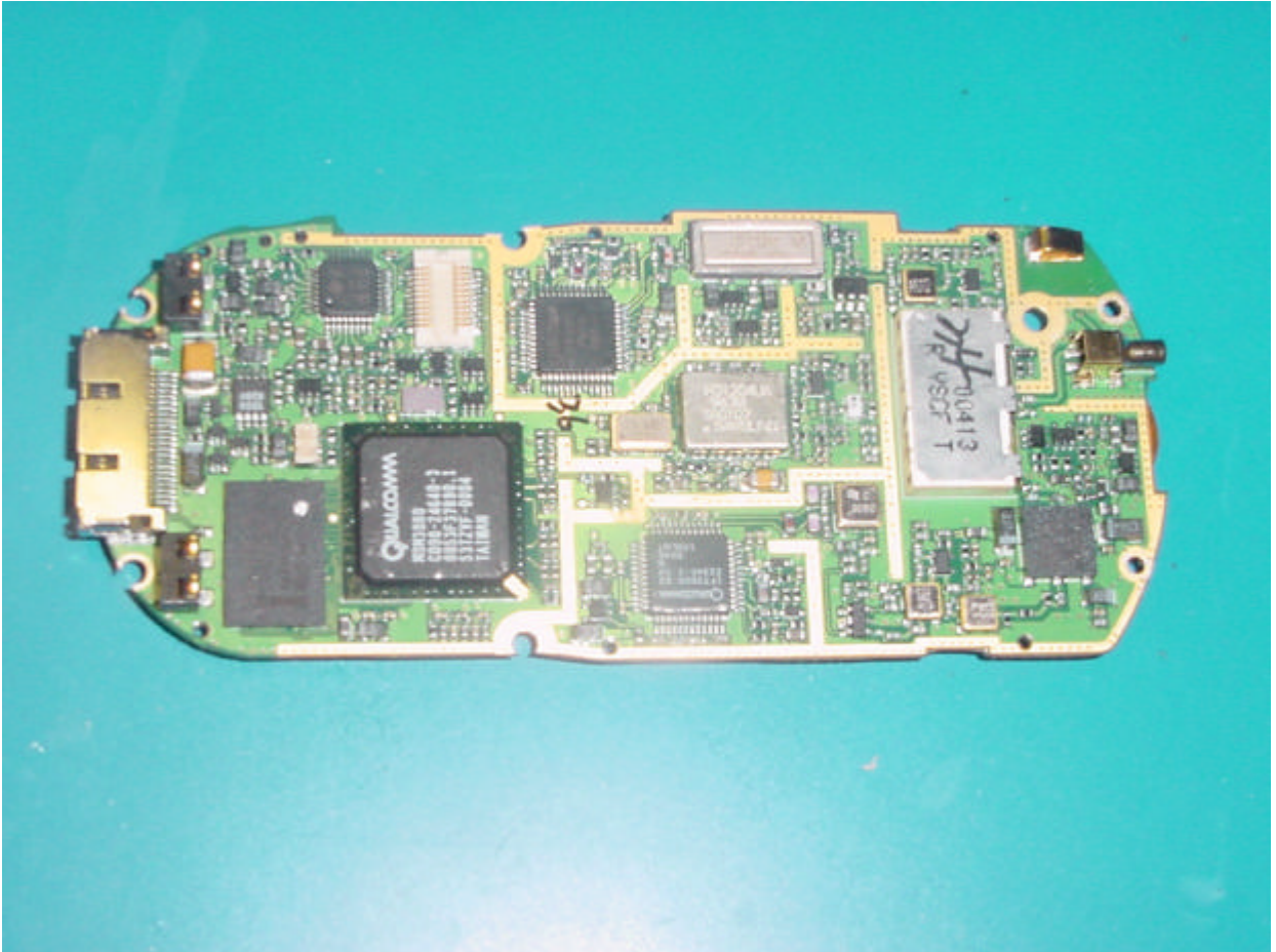
PHOTOGRAPH 11: MAIN BOARD REAR WITH SHIELDS
