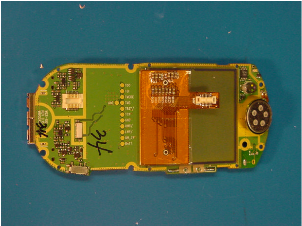
PHOTOGRAPH 10: MAIN BOARD LCD WITH FLIP UP BOARD
