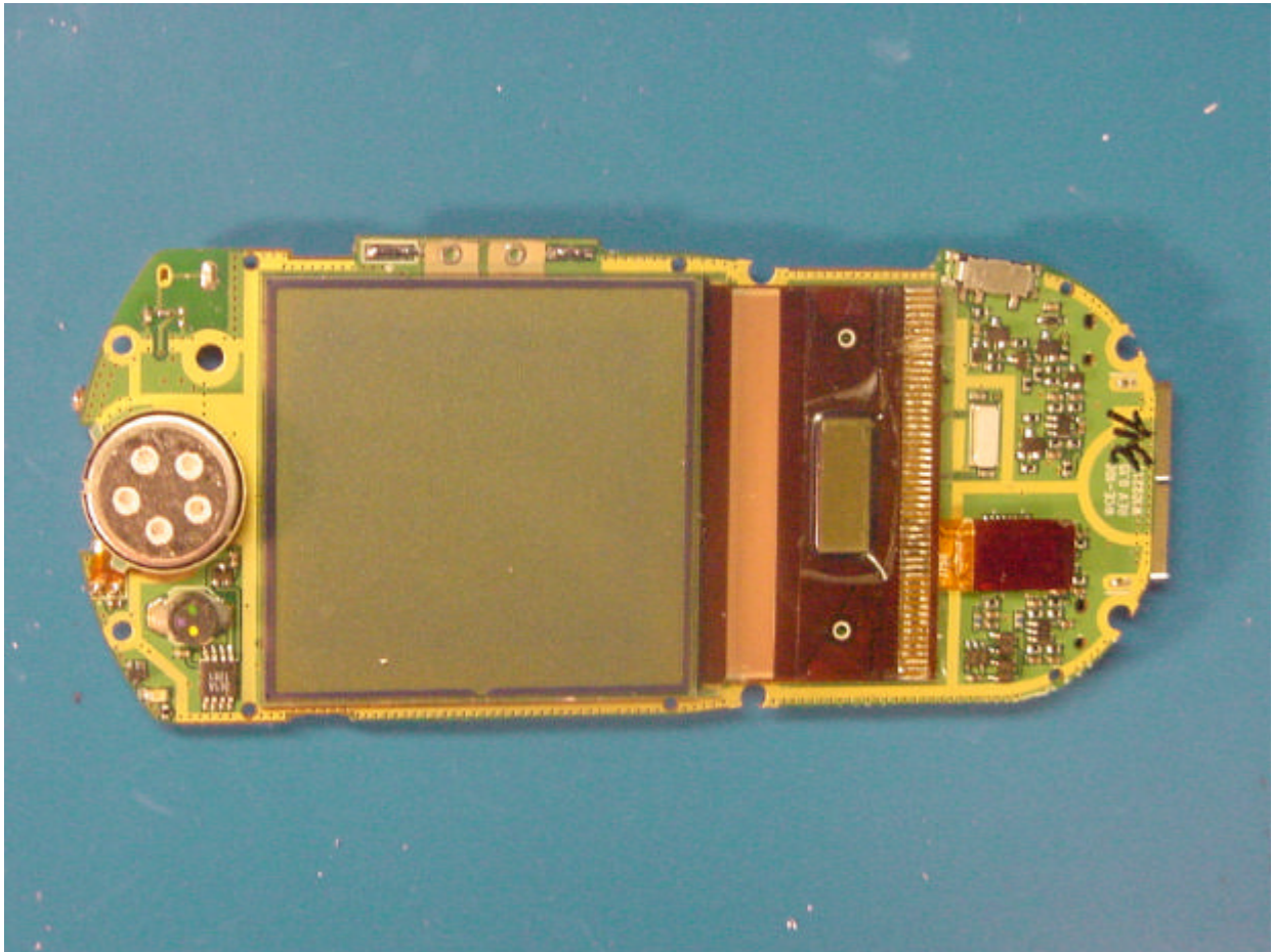
PHOTOGRAPH 9: MAIN BOARD LCD FRONT
