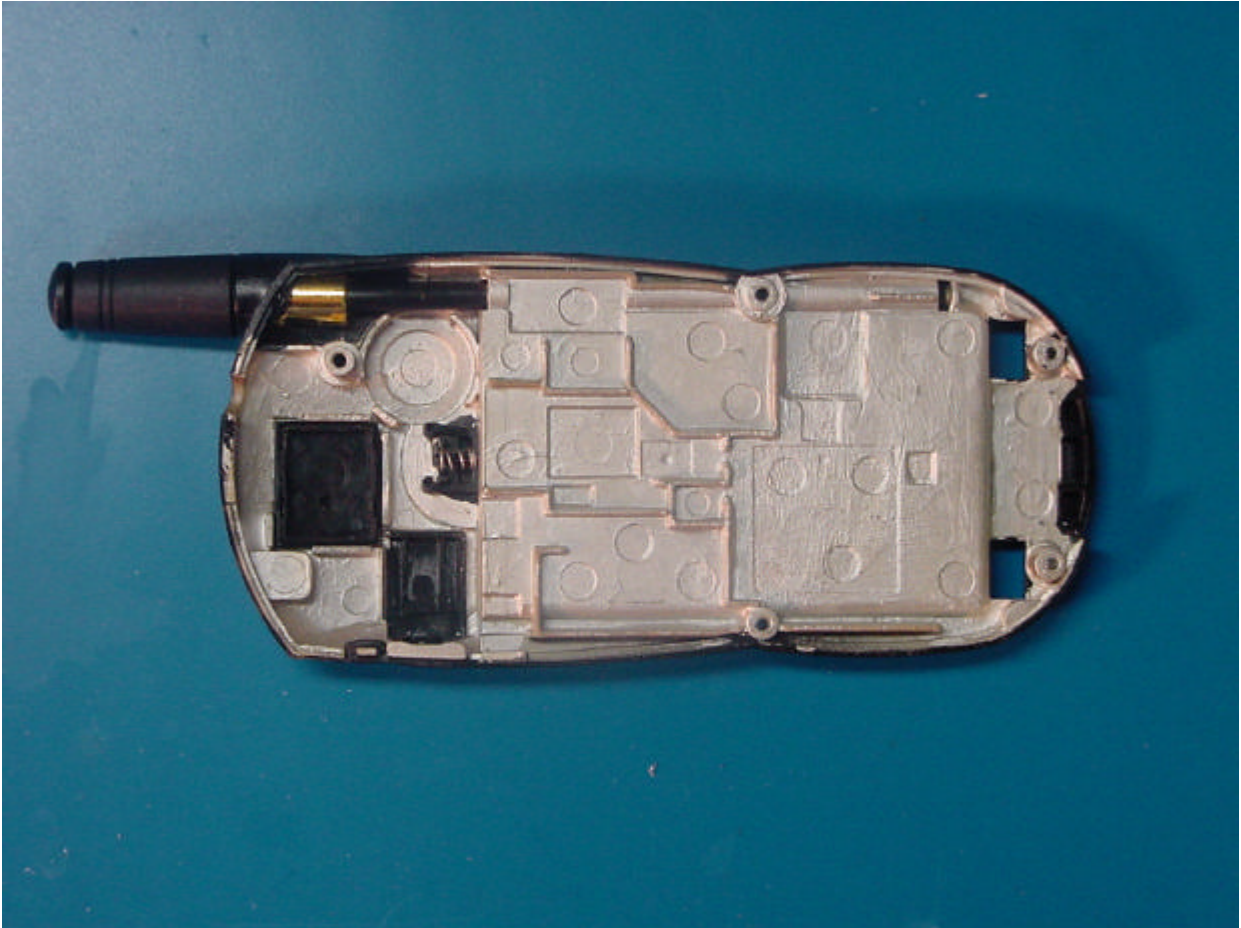
PHOTOGRAPH 6: REAR INSIDE
