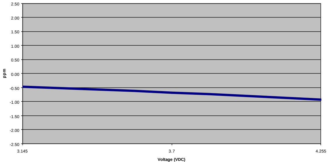
Voltage Frequency Stability (Battery end-point = 2.68 VDC)
