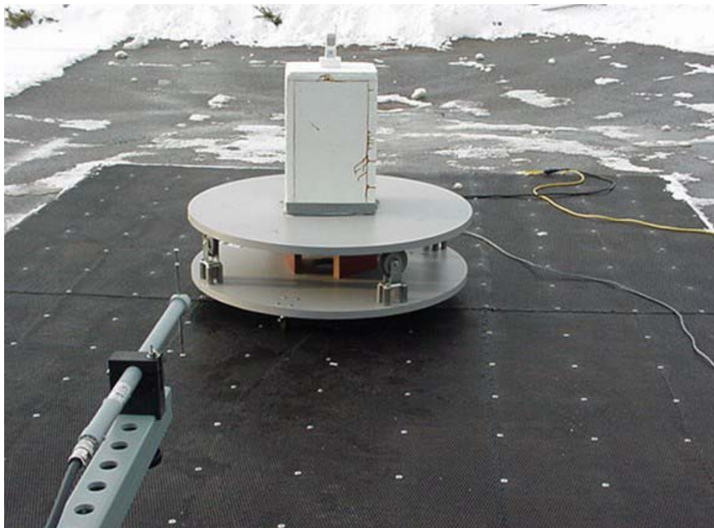
Radiated Measurement Test Setup Photograph
