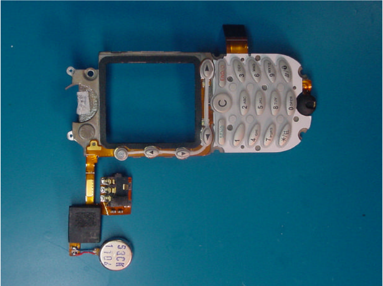
PHOTOGRAPH 9: KEYBOARD FRONT
