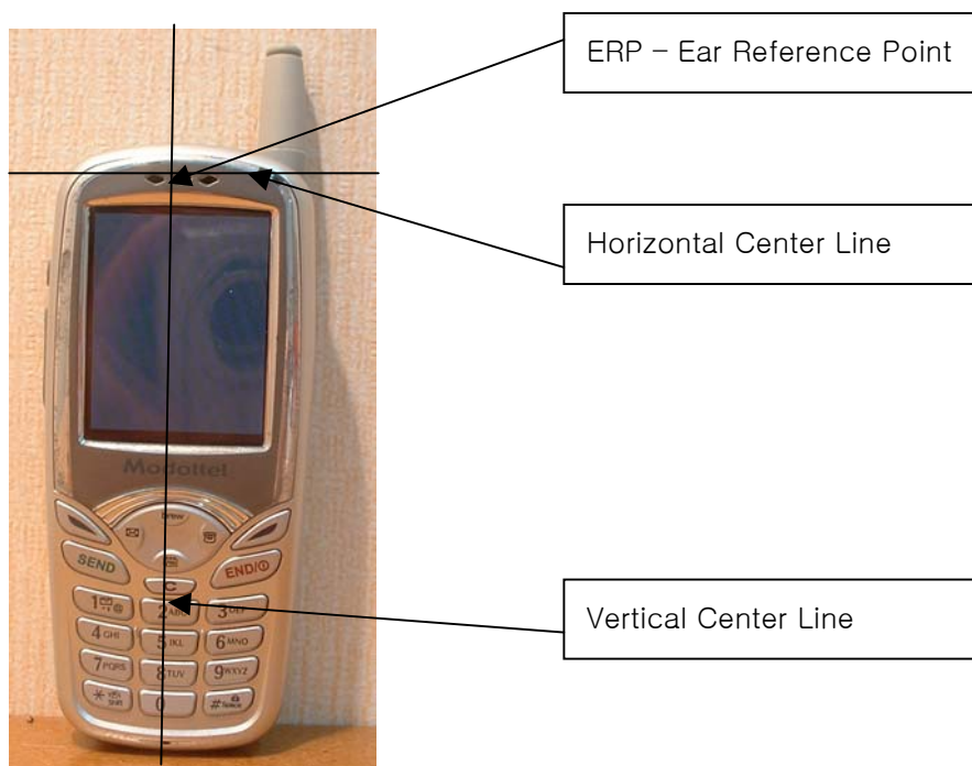
Figure 13.1 handset Reference Points
